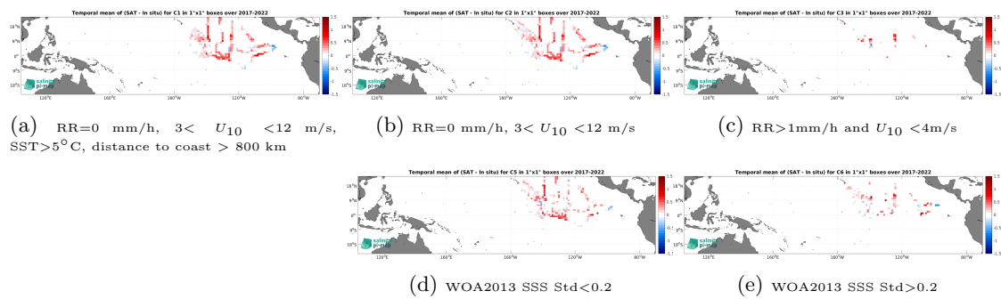
Figure 14: Temporal mean gridded over spatial boxes of size 1^\circ \times 1^\circ of \Delta\text{SSS} (SMOS SSS L4 v1 - Monthly (CMEMS-CNR) - Saildrone) for 5 different subdatasets corresponding to:RR=0 mm/h, 3 < U_{10} < 12 m/s, SST > 5^\circ\text{C} , distance to coast > 800 km (a), RR=0 mm/h, 3 < U_{10} < 12 m/s (b), RR > 1 mm/h and U_{10} < 4 m/s (c), WOA2013 SSS Std < 0.2 (d), WOA2013 SSS Std > 0.2 (e).
