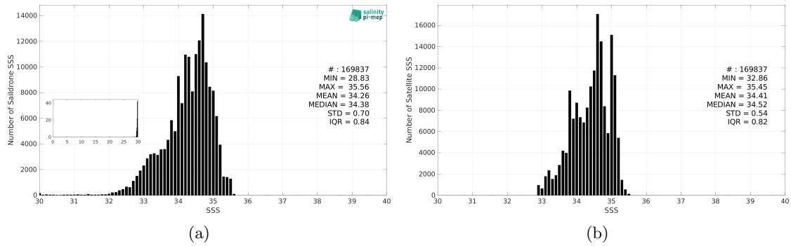
Figure 3: Histograms of SSS from Saildrone (a) and SMOS SSS L4 v1 - Monthly (CMEMS-CNR) (b) considering all match-up pairs per bins of 0.1 over the Tropical Pacific Ocean Pi-MEP region and for the full satellite product period.
