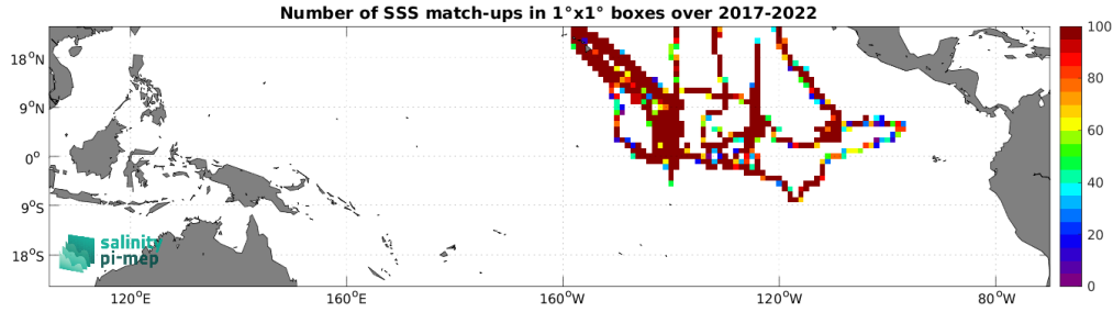
Figure 5: Number of SSS match-ups between Saildrone SSS and the SMOS SSS L4 v1 - Monthly (CMEMS-CNR) SSS product for the Tropical Pacific Ocean Pi-MEP region over 1^\circ \times 1^\circ boxes and for the full satellite product period.
