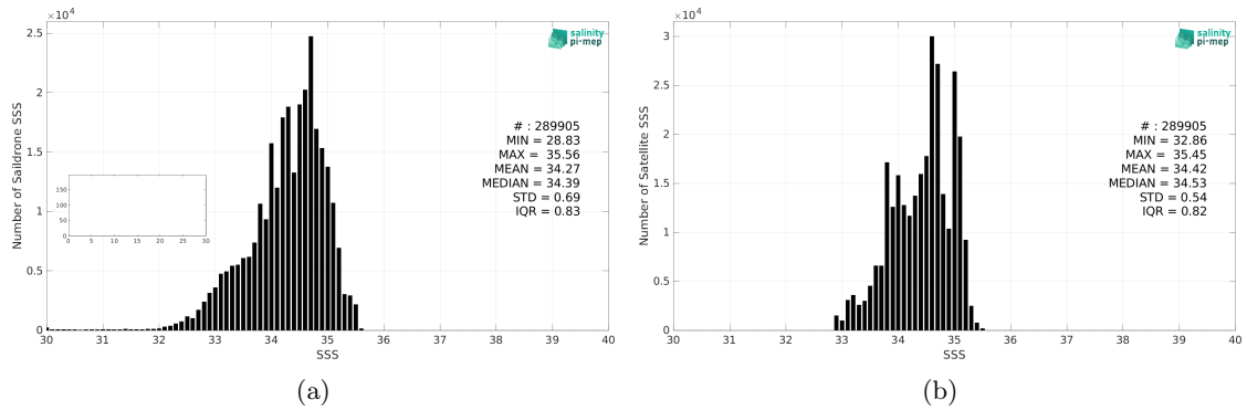
Figure 2: Histograms of SSS from Saildrone (a) and SMOS SSS L4 v1 - Monthly (CMEMS-CNR) (b) considering all match-up pairs per bins of 0.1 over the Tropical Pacific Ocean Pi-MEP region and for the full satellite product period.
