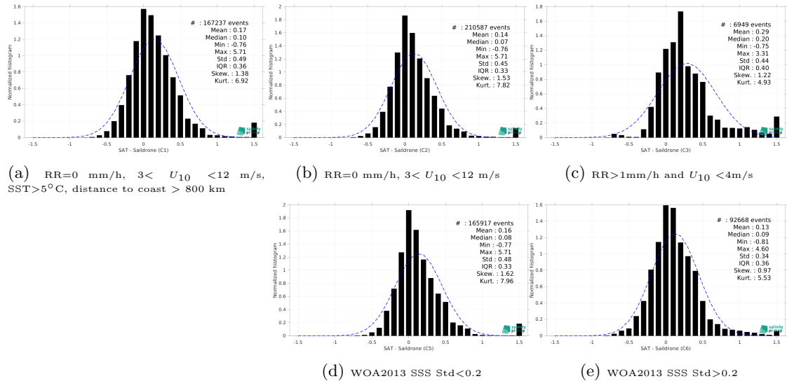
Figure 13: Normalized histogram of \Delta\text{SSS} (SMOS SSS L4 v1 - Monthly (CMEMS-CNR) - Saildrone) for 5 different subdatasets corresponding to: RR=0 mm/h, 3 < U_{10} < 12 m/s, SST >5^\circ\text{C} , distance to coast > 800 km (a), RR=0 mm/h, 3 < U_{10} < 12 m/s (b), RR >1 mm/h and U_{10} < 4 m/s (c), WOA2013 SSS Std <0.2 (d), WOA2013 SSS Std >0.2 (e).
