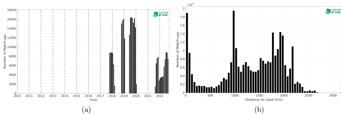
Figure 1: Number of match-ups between Saildrone and SMOS SSS L4 v1 - Monthly (CMEMS-CNR) SSS as a function of time (a) and as function of the distance to coast (b) over the Tropical Pacific Ocean Pi-MEP region and for the full satellite product period.
