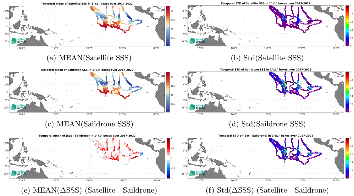
Figure 6: Temporal mean (left) and Std (right) of SSS from SMOS SSS L4 v1 - Monthly (CMEMS-CNR) (top), Saildrone (middle), and of \Delta SSS (Satellite - Saildrone). Only match-up pairs are used to generate these maps.
