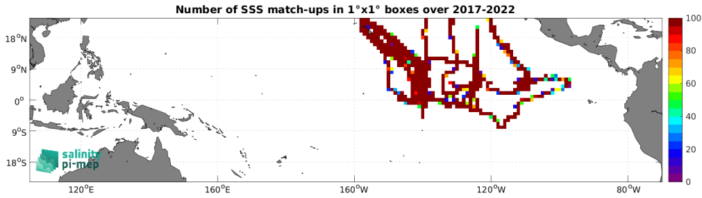
Figure 4: Number of SSS match-ups between Saildrone SSS and the SMOS SSS L4 v1 - Monthly (CMEMS-CNR) SSS product for the Tropical Pacific Ocean Pi-MEP region over 1^\circ \times 1^\circ boxes and for the full satellite product period.
