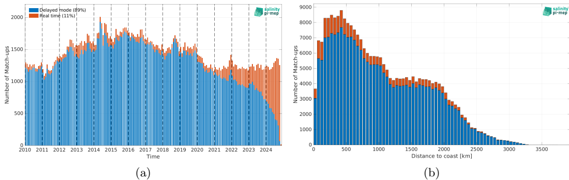
Figure 2: Number of match-ups between Argo and SMOS SSS L4 v1 - Monthly (CMEMS-CNR) SSS as a function of time (a) and as function of the distance to coast (b) over the Tropical Pacific Ocean Pi-MEP region and for the full satellite product period.
