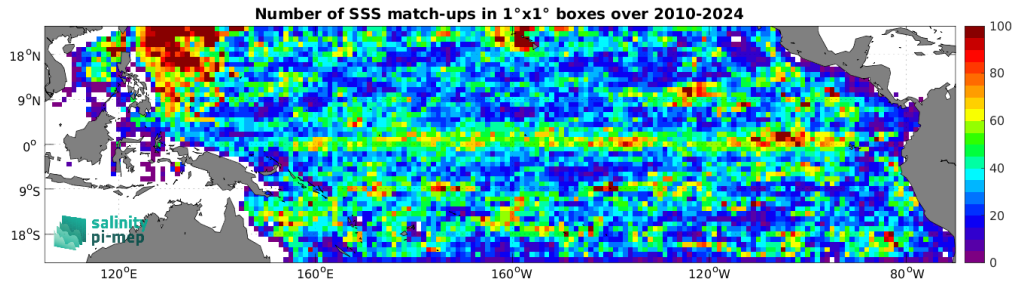
Figure 5: Number of SSS match-ups between Argo SSS and the SMOS SSS L4 v1 - Monthly (CMEMS-CNR) SSS product for the Tropical Pacific Ocean Pi-MEP region over 1^\circ \times 1^\circ boxes and for the full satellite product period.
