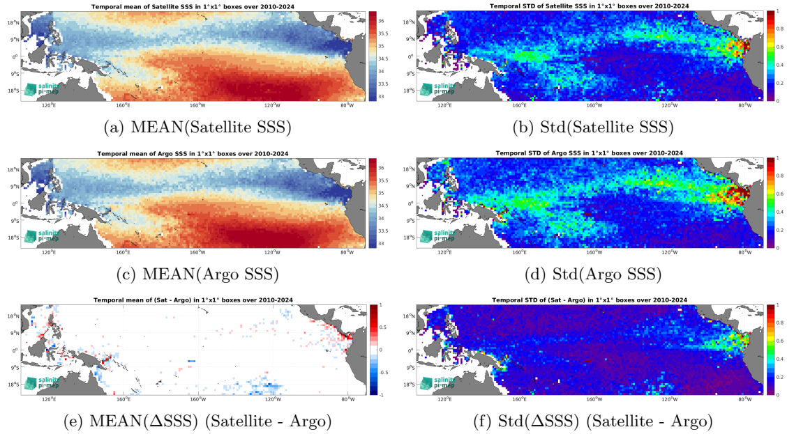
Figure 7: Temporal mean (left) and Std (right) of SSS from SMOS SSS L4 v1 - Monthly (CMEMS-CNR) (top), Argo (middle), and of \Delta SSS (Satellite - Argo). Only match-up pairs are used to generate these maps.
