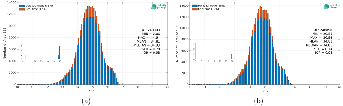
Figure 3: Histograms of SSS from Argo (a) and SMOS SSS L4 v1 - Monthly (CMEMS-CNR) (b) considering all match-up pairs per bins of 0.1 over the Tropical Pacific Ocean Pi-MEP region and for the full satellite product period.
