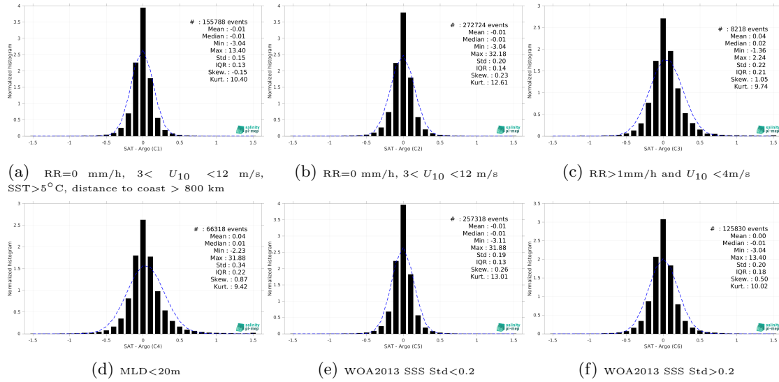
Figure 13: Normalized histogram of \Delta SSS (SMOS SSS L4 v1 - Monthly (CMEMS-CNR) - Argo) for 6 different subdatasets corresponding to: RR=0 mm/h, 3 < U_{10} < 12 m/s, SST > 5°C, distance to coast > 800 km (a), RR=0 mm/h, 3 < U_{10} < 12 m/s (b), RR > 1mm/h and U_{10} < 4 m/s (c), MLD < 20m (d), WOA2013 SSS Std < 0.2 (e), WOA2013 SSS Std > 0.2 (f).
