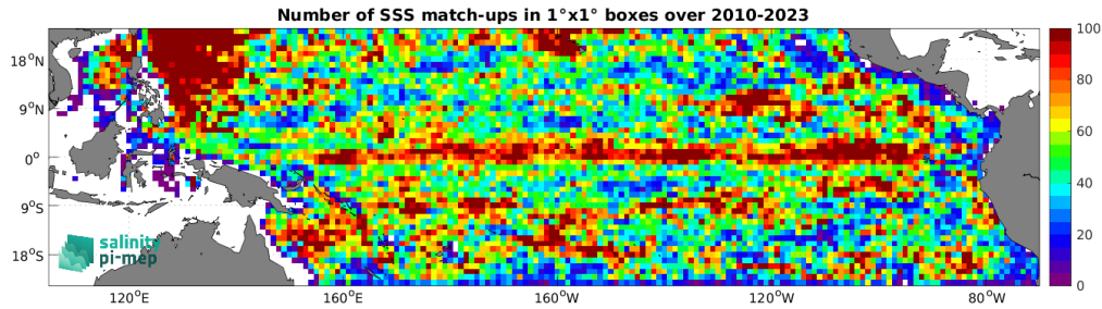
Figure 4: Number of SSS match-ups between Argo SSS and the SMOS SSS L4 v1 - Monthly (CMEMS-CNR) SSS product for the Tropical Pacific Ocean Pi-MEP region over 1^\circ \times 1^\circ boxes and for the full satellite product period.
