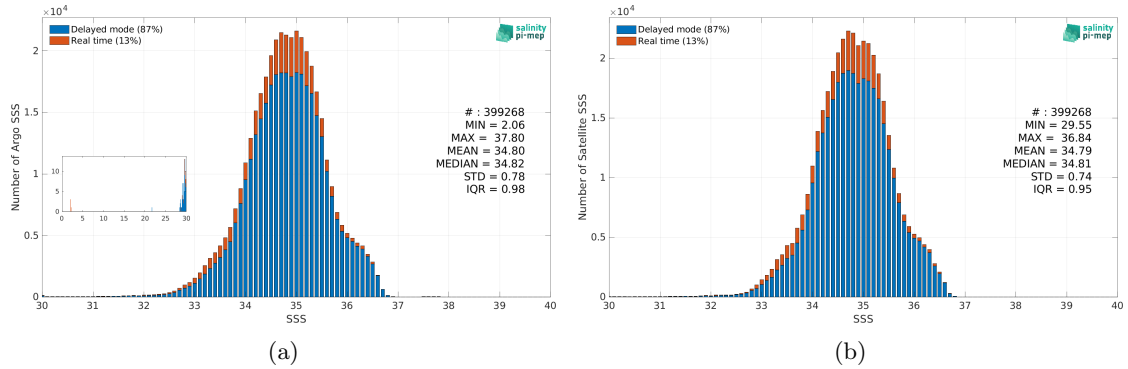
Figure 2: Histograms of SSS from Argo (a) and SMOS SSS L4 v1 - Monthly (CMEMS-CNR) (b) considering all match-up pairs per bins of 0.1 over the Tropical Pacific Ocean Pi-MEP region and for the full satellite product period.
