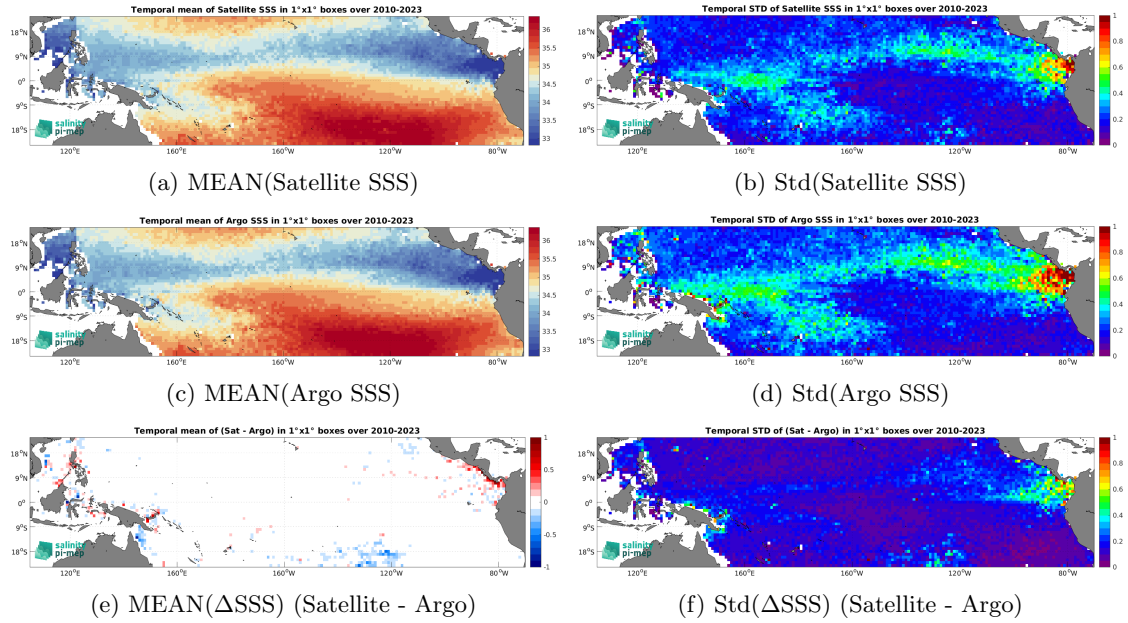
Figure 6: Temporal mean (left) and Std (right) of SSS from SMOS SSS L4 v1 - Monthly (CMEMS-CNR) (top), Argo (middle), and of \Delta SSS (Satellite - Argo). Only match-up pairs are used to generate these maps.
