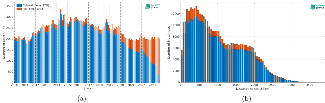
Figure 1: Number of match-ups between Argo and SMOS SSS L4 v1 - Monthly (CMEMS-CNR) SSS as a function of time (a) and as function of the distance to coast (b) over the Tropical Pacific Ocean Pi-MEP region and for the full satellite product period.
