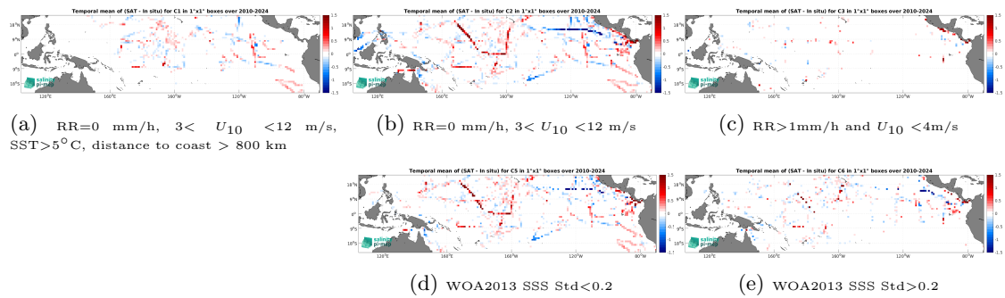
Figure 14: Temporal mean gridded over spatial boxes of size 1^\circ \times 1^\circ of \Delta SSS (SMOS SSS L4 v1 - Daily (CMEMS-CNR) - TSG (SAMOS)) for 5 different subdatasets corresponding to:RR=0 mm/h, 3 < U_{10} < 12 m/s, SST > 5^\circ\text{C} , distance to coast > 800 km (a), RR=0 mm/h, 3 < U_{10} < 12 m/s (b), RR > 1 mm/h and U_{10} < 4 m/s (c), WOA2013 SSS Std < 0.2 (d), WOA2013 SSS Std > 0.2 (e).
