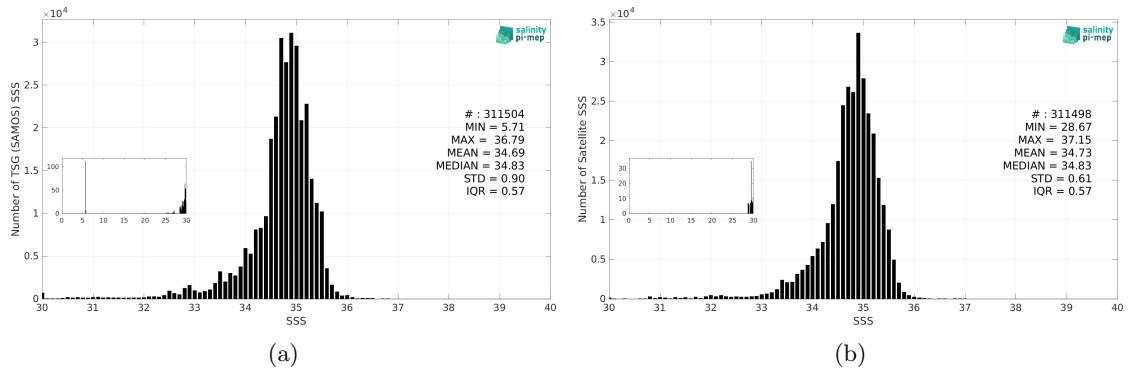
Figure 3: Histograms of SSS from TSG (SAMOS) (a) and SMOS SSS L4 v1 - Daily (CMEMS-CNR) (b) considering all match-up pairs per bins of 0.1 over the Tropical Pacific Ocean Pi-MEP region and for the full satellite product period.
