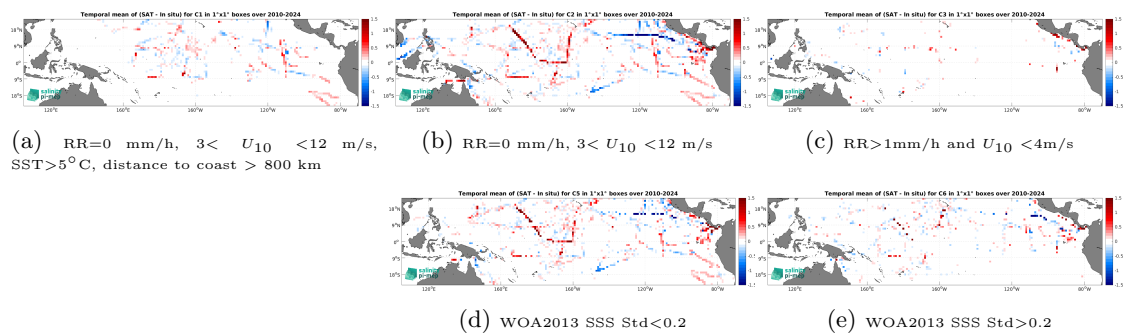
Figure 14: Temporal mean gridded over spatial boxes of size 1^\circ \times 1^\circ of \Delta SSS (SMOS SSS L4 v1 - Daily (CMEMS-CNR) - TSG (SAMOS)) for 5 different subdatasets corresponding to: RR=0 mm/h, 3 < U_{10} < 12 m/s, SST > 5°C, distance to coast > 800 km (a), RR=0 mm/h, 3 < U_{10} < 12 m/s (b), RR > 1mm/h and U_{10} < 4 m/s (c), WOA2013 SSS Std < 0.2 (d), WOA2013 SSS Std > 0.2 (e).
