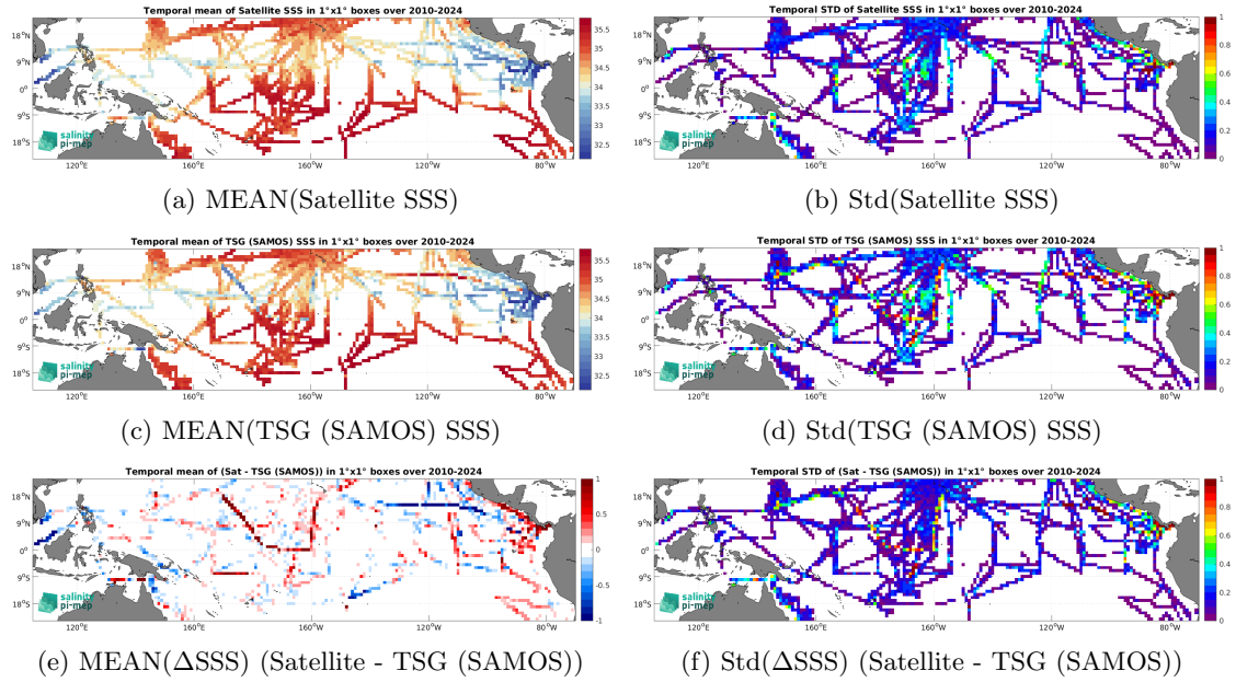
Figure 7: Temporal mean (left) and Std (right) of SSS from SMOS SSS L4 v1 - Daily (CMEMS-CNR) (top), TSG (SAMOS) (middle), and of \Delta SSS (Satellite - TSG (SAMOS)). Only match-up pairs are used to generate these maps.
