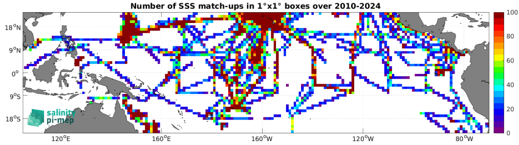
Figure 5: Number of SSS match-ups between TSG (SAMOS) SSS and the SMOS SSS L4 v1 - Daily (CMEMS-CNR) SSS product for the Tropical Pacific Ocean Pi-MEP region over 1^\circ \times 1^\circ boxes and for the full satellite product period.
