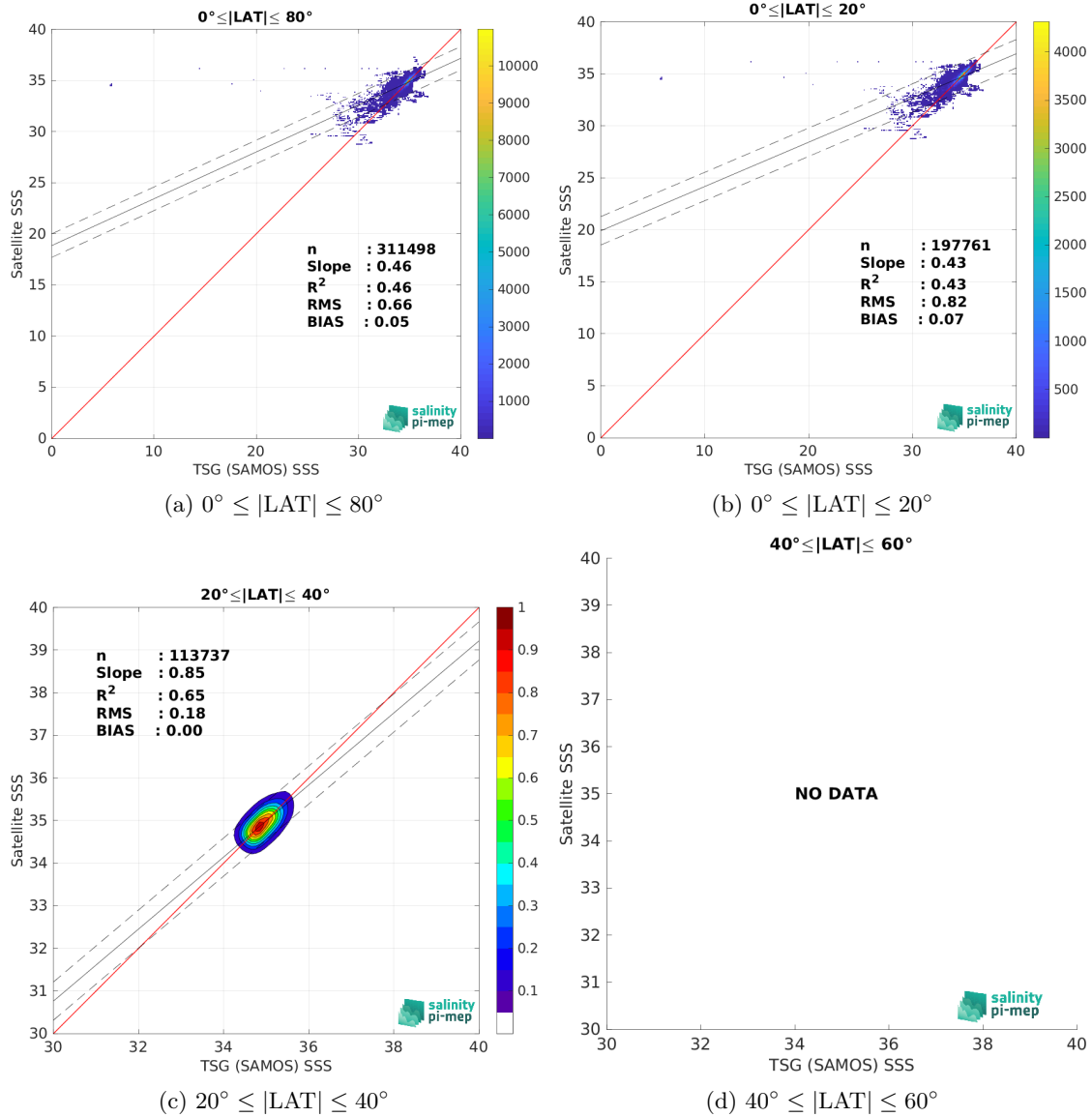
Figure 10: Contour maps of the concentration of SMOS SSS L4 v1 - Daily (CMEMS-CNR) SSS (y-axis) versus TSG (SAMOS) SSS (x-axis) at match-up pairs for different latitude bands. For each plot, the red line shows x=y . The black thin and dashed lines indicate a linear fit through the data cloud and the \pm 95\% confidence levels, respectively. The number match-up pairs n , the slope and R^2 coefficient of the linear fit, the root mean square (RMS) and the mean bias between satellite and in situ data are indicated for each latitude band in each plots.
