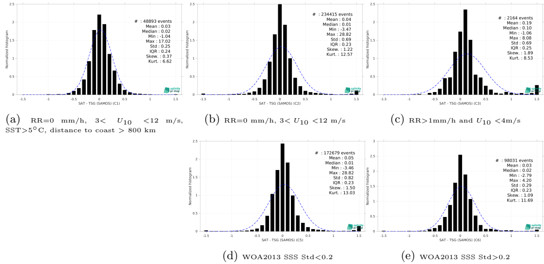
Figure 15: Normalized histogram of \Delta\text{SSS} (SMOS SSS L4 v1 - Daily (CMEMS-CNR) - TSG (SAMOS)) for 5 different subdatasets corresponding to: RR=0 mm/h, 3 < U_{10} < 12 m/s, SST>5°C, distance to coast > 800 km (a), RR=0 mm/h, 3 < U_{10} < 12 m/s (b), RR>1mm/h and U_{10} < 4 m/s (c), WOA2013 SSS Std<0.2 (d), WOA2013 SSS Std>0.2 (e).
