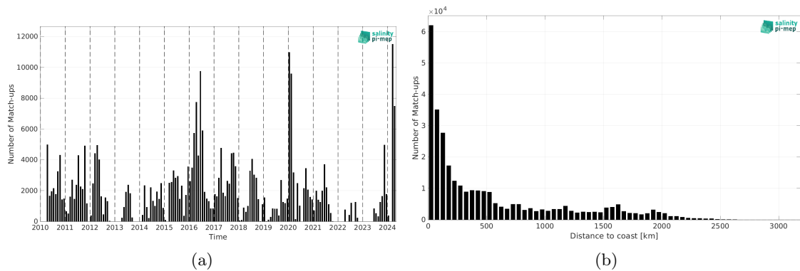
Figure 2: Number of match-ups between TSG (SAMOS) and SMOS SSS L4 v1 - Daily (CMEMS-CNR) SSS as a function of time (a) and as function of the distance to coast (b) over the Tropical Pacific Ocean Pi-MEP region and for the full satellite product period.
