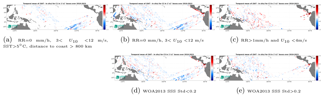
Figure 14: Temporal mean gridded over spatial boxes of size 1^\circ \times 1^\circ of \Delta SSS (SMOS SSS L4 v1 - Daily (CMEMS-CNR) - TSG (LEGOS-DM)) for 5 different subdatasets corresponding to: RR=0 mm/h, 3 < U_{10} < 12 m/s, SST > 5°C, distance to coast > 800 km (a), RR=0 mm/h, 3 < U_{10} < 12 m/s (b), RR > 1mm/h and U_{10} < 4 m/s (c), WOA2013 SSS Std < 0.2 (d), WOA2013 SSS Std > 0.2 (e).
