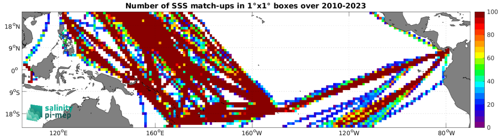
Figure 5: Number of SSS match-ups between TSG (LEGOS-DM) SSS and the SMOS SSS L4 v1 - Daily (CMEMS-CNR) SSS product for the Tropical Pacific Ocean Pi-MEP region over 1^\circ \times 1^\circ boxes and for the full satellite product period.
