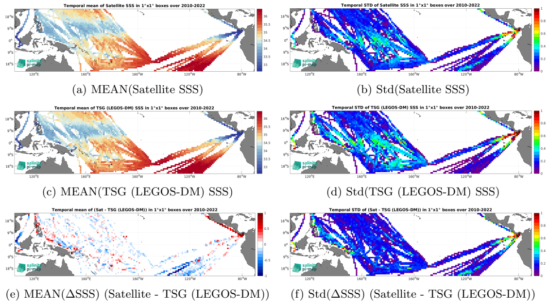
Figure 7: Temporal mean (left) and Std (right) of SSS from SMOS SSS L4 v1 - Daily (CMEMS-CNR) (top), TSG (LEGOS-DM) (middle), and of \Delta SSS (Satellite - TSG (LEGOS-DM)). Only match-up pairs are used to generate these maps.
