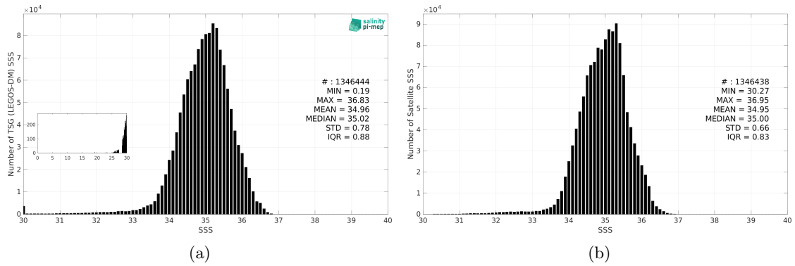
Figure 3: Histograms of SSS from TSG (LEGOS-DM) (a) and SMOS SSS L4 v1 - Daily (CMEMS-CNR) (b) considering all match-up pairs per bins of 0.1 over the Tropical Pacific Ocean Pi-MEP region and for the full satellite product period.
