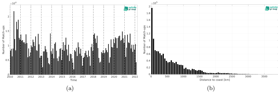
Figure 2: Number of match-ups between TSG (LEGOS-DM) and SMOS SSS L4 v1 - Daily (CMEMS-CNR) SSS as a function of time (a) and as function of the distance to coast (b) over the Tropical Pacific Ocean Pi-MEP region and for the full satellite product period.
