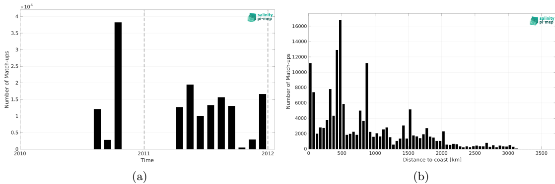
Figure 2: Number of match-ups between TSG (GOSUD-Sailing-ship) and SMOS SSS L4 v1 - Daily (CMEMS-CNR) SSS as a function of time (a) and as function of the distance to coast (b) over the Tropical Pacific Ocean Pi-MEP region and for the full satellite product period.
