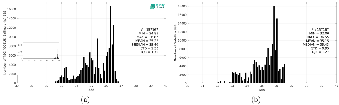
Figure 3: Histograms of SSS from TSG (GOSUD-Sailing-ship) (a) and SMOS SSS L4 v1 - Daily (CMEMS-CNR) (b) considering all match-up pairs per bins of 0.1 over the Tropical Pacific Ocean Pi-MEP region and for the full satellite product period.
