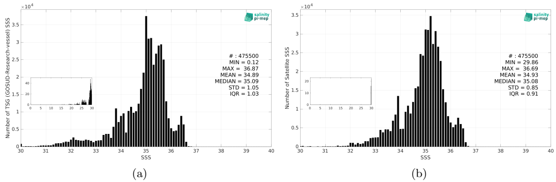
Figure 3: Histograms of SSS from TSG (GOSUD-Research-vessel) (a) and SMOS SSS L4 v1 - Daily (CMEMS-CNR) (b) considering all match-up pairs per bins of 0.1 over the Tropical Pacific Ocean Pi-MEP region and for the full satellite product period.
