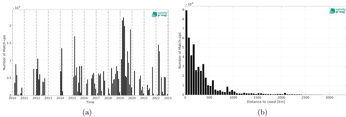
Figure 2: Number of match-ups between TSG (GOSUD-Research-vessel) and SMOS SSS L4 v1 - Daily (CMEMS-CNR) SSS as a function of time (a) and as function of the distance to coast (b) over the Tropical Pacific Ocean Pi-MEP region and for the full satellite product period.
