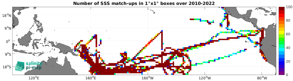
Figure 5: Number of SSS match-ups between TSG (GOSUD-Research-vessel) SSS and the SMOS SSS L4 v1 - Daily (CMEMS-CNR) SSS product for the Tropical Pacific Ocean Pi-MEP region over 1^\circ \times 1^\circ boxes and for the full satellite product period.
