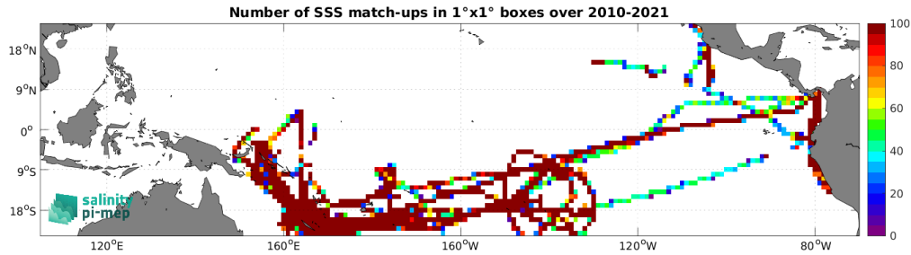
Figure 5: Number of SSS match-ups between TSG (GOSUD-Research-vessel) SSS and the SMOS SSS L4 v1 - Daily (CMEMS-CNR) SSS product for the Tropical Pacific Ocean Pi-MEP region over 1^\circ \times 1^\circ boxes and for the full satellite product period.
