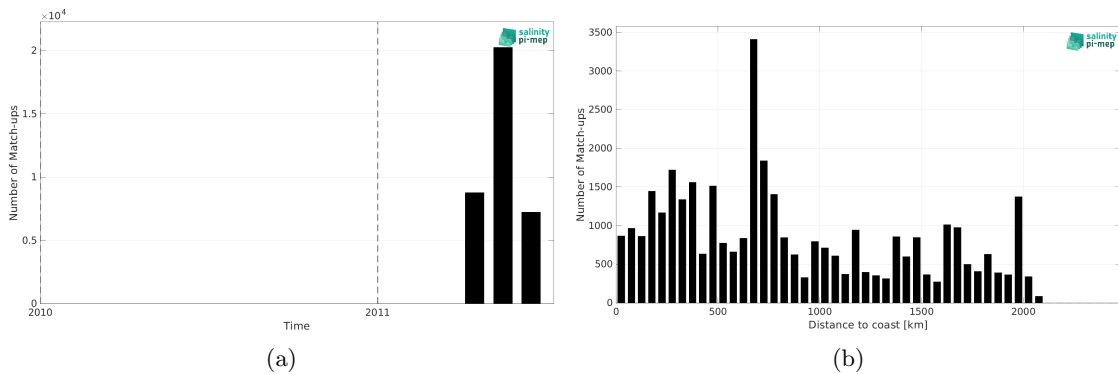
Figure 2: Number of match-ups between TSG (CSIC-UTM) and SMOS SSS L4 v1 - Daily (CMEMS-CNR) SSS as a function of time (a) and as function of the distance to coast (b) over the Tropical Pacific Ocean Pi-MEP region and for the full satellite product period.
