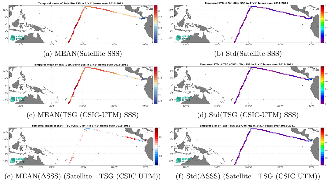
Figure 7: Temporal mean (left) and Std (right) of SSS from SMOS SSS L4 v1 - Daily (CMEMS-CNR) (top), TSG (CSIC-UTM) (middle), and of \Delta SSS (Satellite - TSG (CSIC-UTM)). Only match-up pairs are used to generate these maps.
