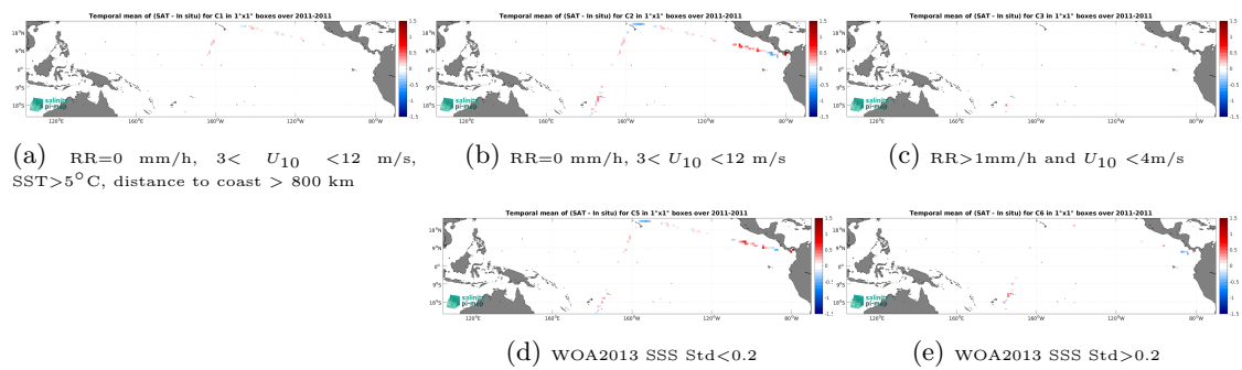
Figure 14: Temporal mean gridded over spatial boxes of size 1^\circ \times 1^\circ of \Delta SSS (SMOS SSS L4 v1 - Daily (CMEMS-CNR) - TSG (CSIC-UTM)) for 5 different subdatasets corresponding to: RR=0 mm/h, 3 < U_{10} < 12 m/s, SST > 5^\circ\text{C} , distance to coast > 800 km (a), RR=0 mm/h, 3 < U_{10} < 12 m/s (b), RR > 1 mm/h and U_{10} < 4 m/s (c), WOA2013 SSS Std < 0.2 (d), WOA2013 SSS Std > 0.2 (e).
