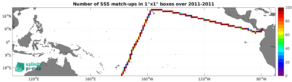
Figure 5: Number of SSS match-ups between TSG (CSIC-UTM) SSS and the SMOS SSS L4 v1 - Daily (CMEMS-CNR) SSS product for the Tropical Pacific Ocean Pi-MEP region over 1^\circ \times 1^\circ boxes and for the full satellite product period.
