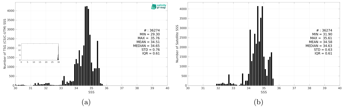
Figure 3: Histograms of SSS from TSG (CSIC-UTM) (a) and SMOS SSS L4 v1 - Daily (CMEMS-CNR) (b) considering all match-up pairs per bins of 0.1 over the Tropical Pacific Ocean Pi-MEP region and for the full satellite product period.
