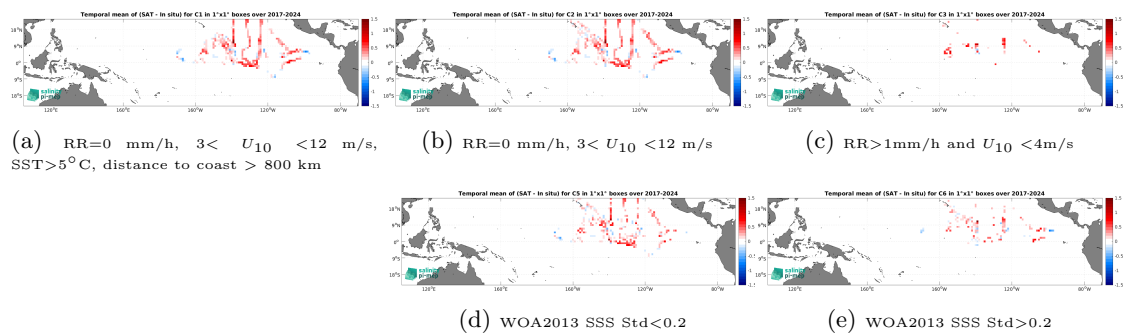
Figure 14: Temporal mean gridded over spatial boxes of size 1^\circ \times 1^\circ of \Delta\text{SSS} (SMOS SSS L4 v1 - Daily (CMEMS-CNR) - Saildrone) for 5 different subdatasets corresponding to: RR=0 mm/h, 3 < U_{10} < 12 m/s, SST > 5°C, distance to coast > 800 km (a), RR=0 mm/h, 3 < U_{10} < 12 m/s (b), RR > 1mm/h and U_{10} < 4 m/s (c), WOA2013 SSS Std < 0.2 (d), WOA2013 SSS Std > 0.2 (e).
