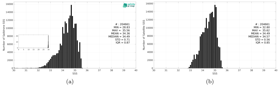
Figure 3: Histograms of SSS from Sairdrone (a) and SMOS SSS L4 v1 - Daily (CMEMS-CNR) (b) considering all match-up pairs per bins of 0.1 over the Tropical Pacific Ocean Pi-MEP region and for the full satellite product period.
