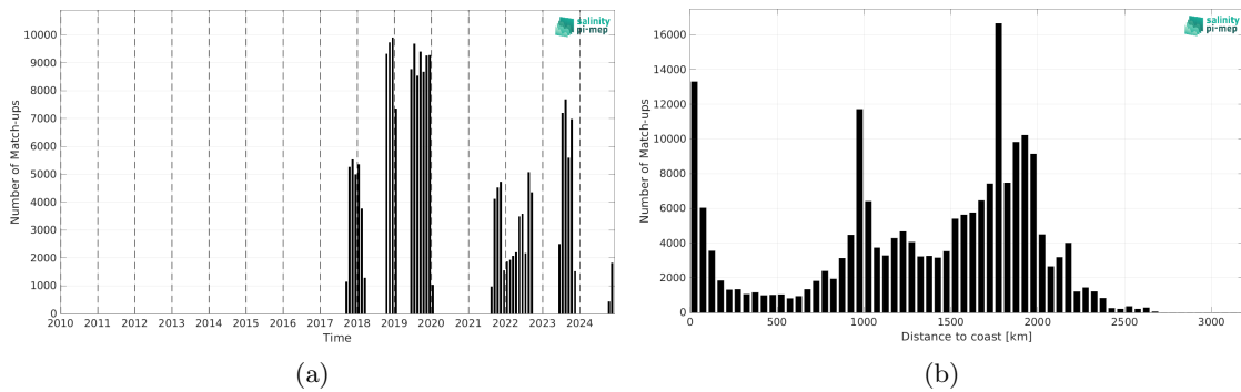
Figure 2: Number of match-ups between Saildrone and SMOS SSS L4 v1 - Daily (CMEMS-CNR) SSS as a function of time (a) and as function of the distance to coast (b) over the Tropical Pacific Ocean Pi-MEP region and for the full satellite product period.
