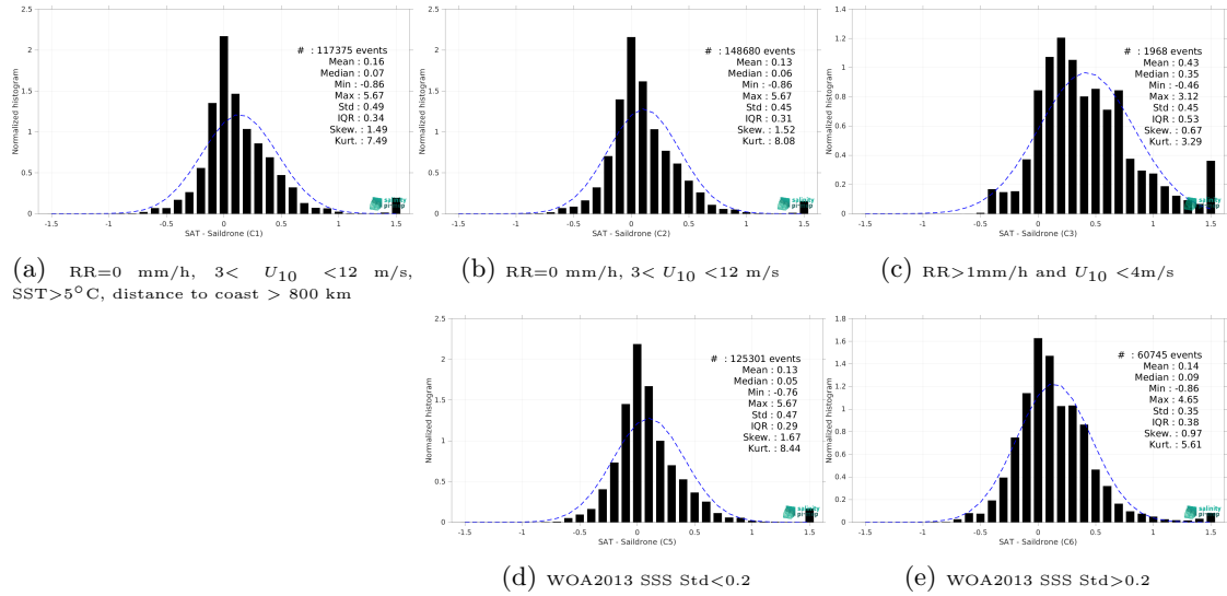
Figure 15: Normalized histogram of \Delta SSS (SMOS SSS L4 v1 - Daily (CMEMS-CNR) - Sairdrone) for 5 different subdatasets corresponding to: RR=0 mm/h, 3 < U_{10} < 12 m/s, SST>5°C, distance to coast > 800 km (a), RR=0 mm/h, 3 < U_{10} < 12 m/s (b), RR>1mm/h and U_{10} < 4 m/s (c), WOA2013 SSS Std<0.2 (d), WOA2013 SSS Std>0.2 (e).
