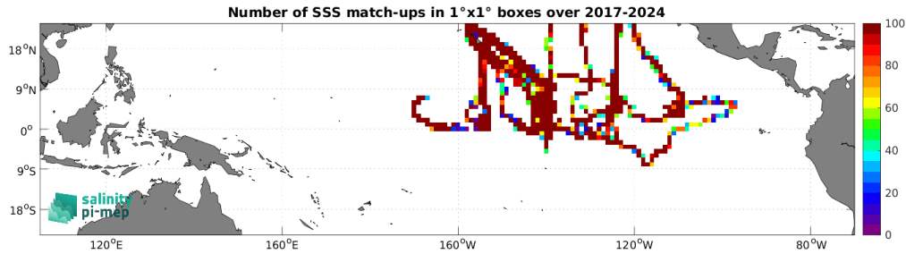
Figure 5: Number of SSS match-ups between Saildrone SSS and the SMOS SSS L4 v1 - Daily (CMEMS-CNR) SSS product for the Tropical Pacific Ocean Pi-MEP region over 1^\circ \times 1^\circ boxes and for the full satellite product period.
