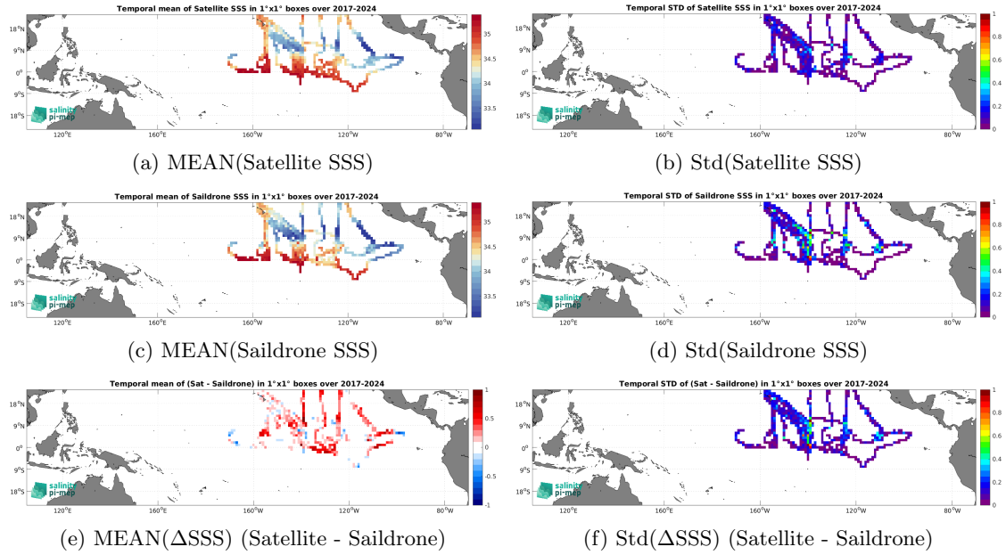
Figure 7: Temporal mean (left) and Std (right) of SSS from SMOS SSS L4 v1 - Daily (CMEMS-CNR) (top), Saildrone (middle), and of \Delta SSS (Satellite - Saildrone). Only match-up pairs are used to generate these maps.
