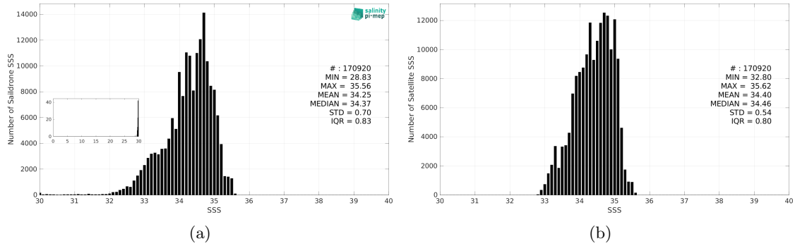
Figure 3: Histograms of SSS from Saildrone (a) and SMOS SSS L4 v1 - Daily (CMEMS-CNR) (b) considering all match-up pairs per bins of 0.1 over the Tropical Pacific Ocean Pi-MEP region and for the full satellite product period.
