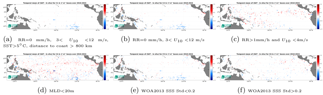
Figure 14: Temporal mean gridded over spatial boxes of size 1^\circ \times 1^\circ of \Delta\text{SSS} (SMOS SSS L4 v1 - Daily (CMEMS-CNR) - Argo) for 6 different subdatasets corresponding to:RR=0 mm/h, 3 < U_{10} < 12 m/s, \text{SST} > 5^\circ\text{C} , distance to coast > 800 km (a), RR=0 mm/h, 3 < U_{10} < 12 m/s (b), RR>1mm/h and U_{10} < 4 m/s (c),MLD<20m (d),WOA2013 SSS Std<0.2 (e),WOA2013 SSS Std>0.2 (f).
