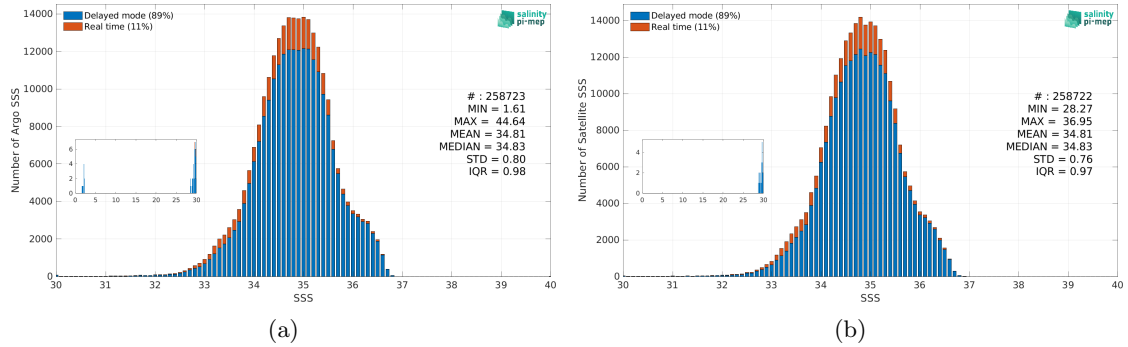
Figure 3: Histograms of SSS from Argo (a) and SMOS SSS L4 v1 - Daily (CMEMS-CNR) (b) considering all match-up pairs per bins of 0.1 over the Tropical Pacific Ocean Pi-MEP region and for the full satellite product period.
