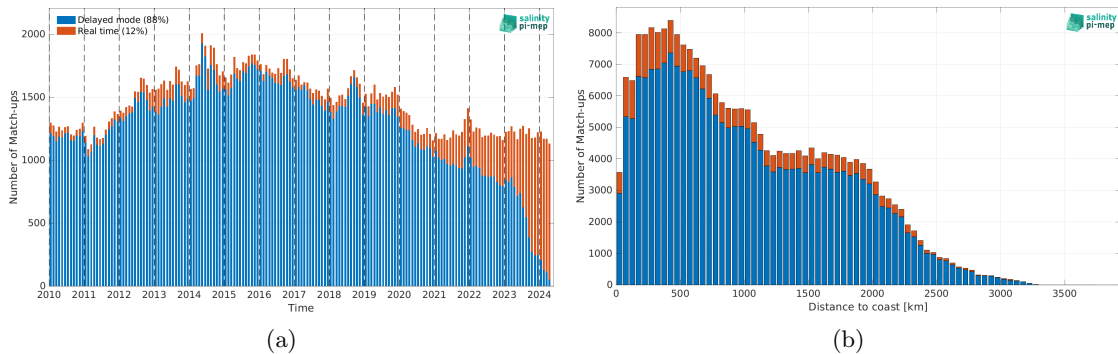
Figure 2: Number of match-ups between Argo and SMOS SSS L4 v1 - Daily (CMEMS-CNR) SSS as a function of time (a) and as function of the distance to coast (b) over the Tropical Pacific Ocean Pi-MEP region and for the full satellite product period.
