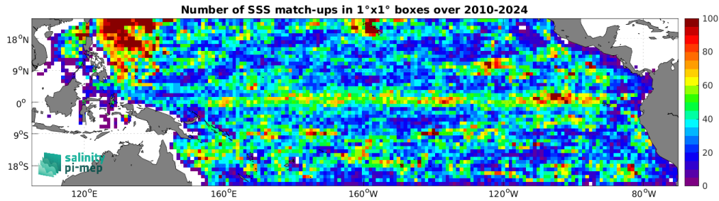
Figure 5: Number of SSS match-ups between Argo SSS and the SMOS SSS L4 v1 - Daily (CMEMS-CNR) SSS product for the Tropical Pacific Ocean Pi-MEP region over 1^\circ \times 1^\circ boxes and for the full satellite product period.
