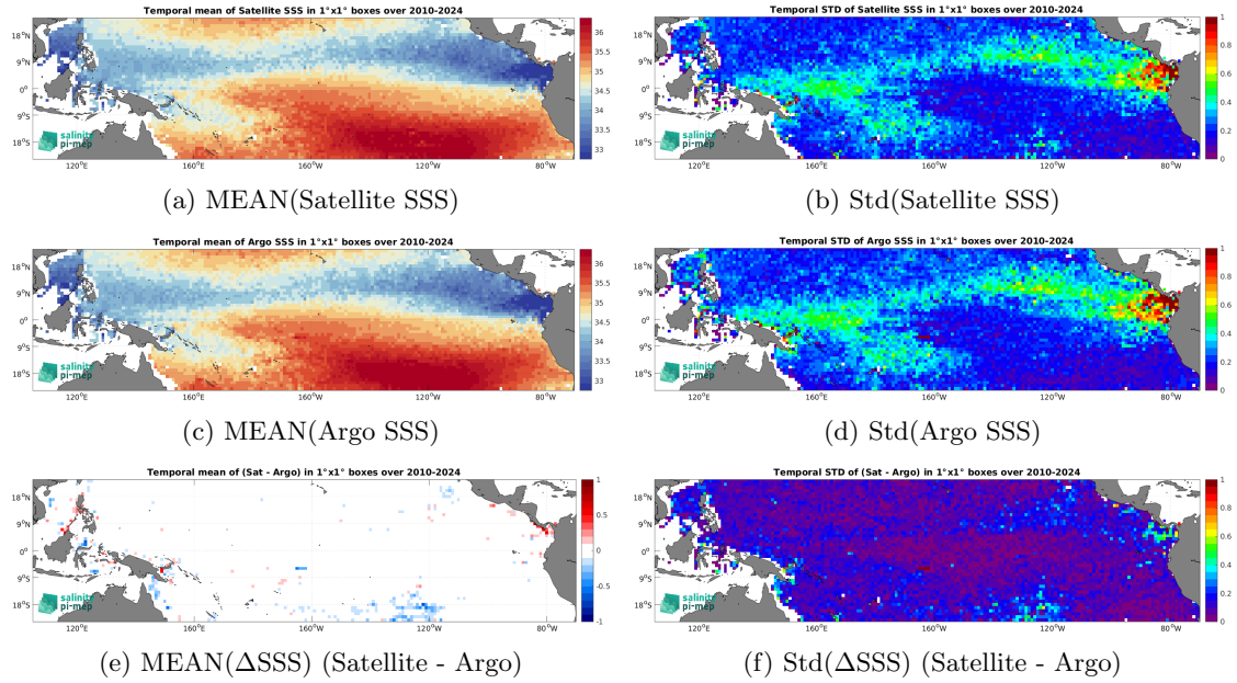
Figure 7: Temporal mean (left) and Std (right) of SSS from SMOS SSS L4 v1 - Daily (CMEMS-CNR) (top), Argo (middle), and of \Delta SSS (Satellite - Argo). Only match-up pairs are used to generate these maps.
