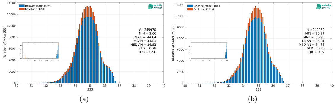
Figure 3: Histograms of SSS from Argo (a) and SMOS SSS L4 v1 - Daily (CMEMS-CNR) (b) considering all match-up pairs per bins of 0.1 over the Tropical Pacific Ocean Pi-MEP region and for the full satellite product period.
