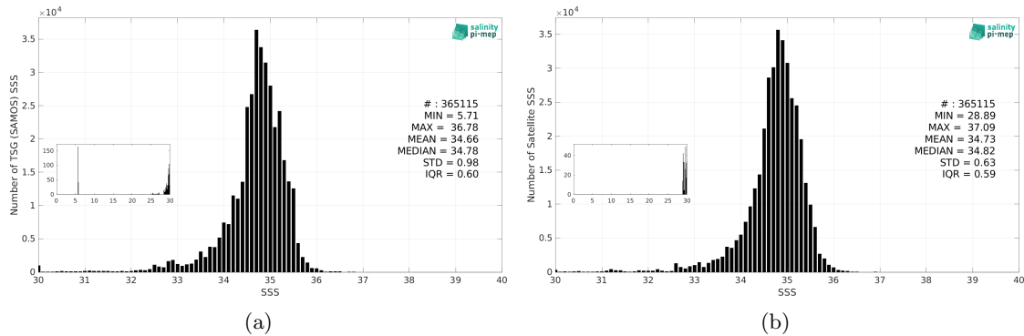
Figure 3: Histograms of SSS from TSG (SAMOS) (a) and SMOS SSS L4 OI v346 - Weekly (CMEMS-CATDS-LOPS) (b) considering all match-up pairs per bins of 0.1 over the Tropical Pacific Ocean Pi-MEP region and for the full satellite product period.
