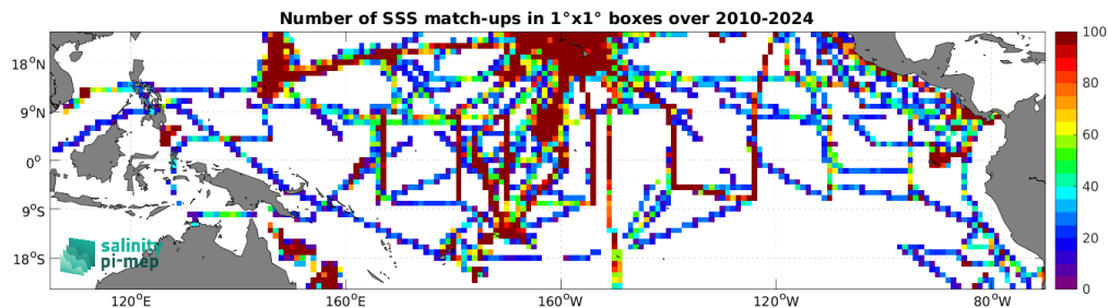
Figure 5: Number of SSS match-ups between TSG (SAMOS) SSS and the SMOS SSS L4 OI v346 - Weekly (CMEMS-CATDS-LOPS) SSS product for the Tropical Pacific Ocean Pi-MEP region over 1^\circ \times 1^\circ boxes and for the full satellite product period.
