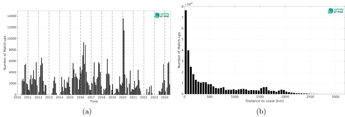
Figure 2: Number of match-ups between TSG (SAMOS) and SMOS SSS L4 OI v346 - Weekly (CMEMS-CATDS-LOPS) SSS as a function of time (a) and as function of the distance to coast (b) over the Tropical Pacific Ocean Pi-MEP region and for the full satellite product period.
