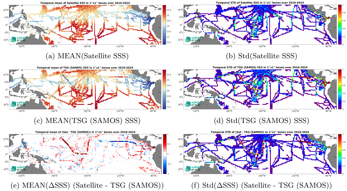
Figure 7: Temporal mean (left) and Std (right) of SSS from SMOS SSS L4 OI v346 - Weekly (CMEMS-CATDS-LOPS) (top), TSG (SAMOS) (middle), and of \Delta SSS (Satellite - TSG (SAMOS)). Only match-up pairs are used to generate these maps.
