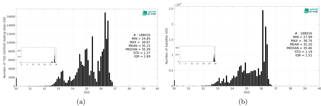
Figure 3: Histograms of SSS from TSG (GOSUD-Sailing-ship) (a) and SMOS SSS L4 OI v346 - Weekly (CMEMS-CATDS-LOPS) (b) considering all match-up pairs per bins of 0.1 over the Tropical Pacific Ocean Pi-MEP region and for the full satellite product period.
