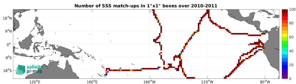
Figure 5: Number of SSS match-ups between TSG (GOSUD-Sailing-ship) SSS and the SMOS SSS L4 OI v346 - Weekly (CMEMS-CATDS-LOPS) SSS product for the Tropical Pacific Ocean Pi-MEP region over 1^\circ \times 1^\circ boxes and for the full satellite product period.
