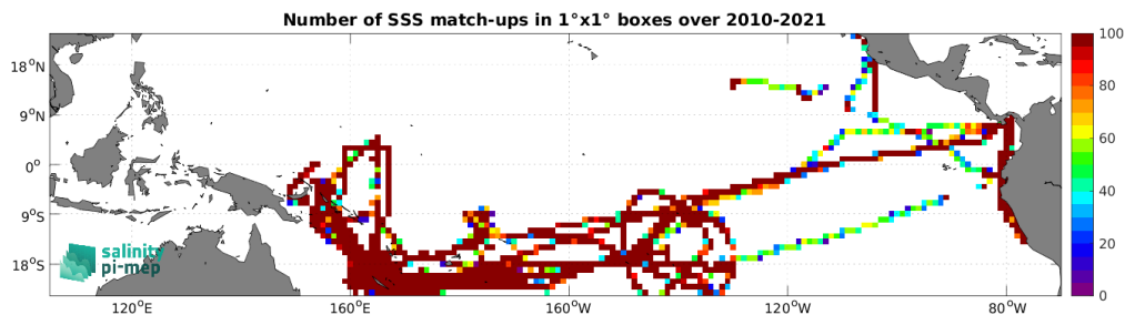
Figure 5: Number of SSS match-ups between TSG (GOSUD-Research-vessel) SSS and the SMOS SSS L4 OI v346 - Weekly (CMEMS-CATDS-LOPS) SSS product for the Tropical Pacific Ocean Pi-MEP region over 1^\circ \times 1^\circ boxes and for the full satellite product period.
