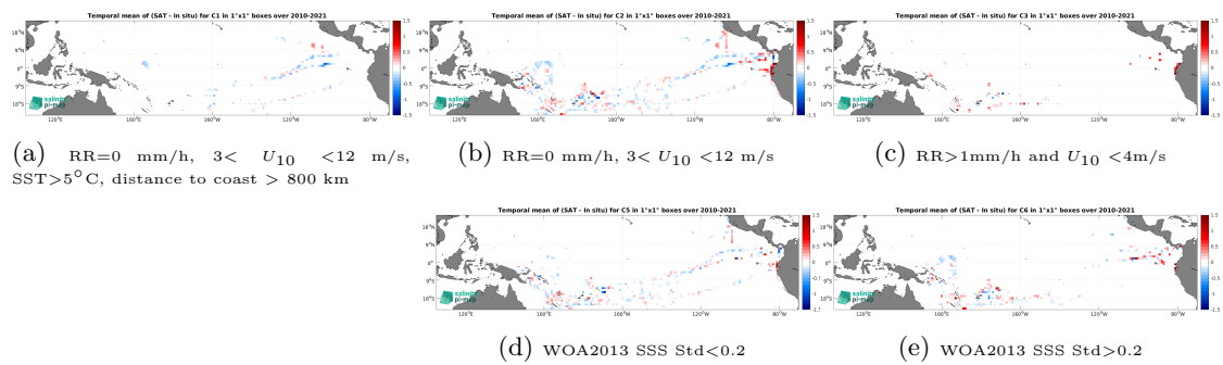
Figure 14: Temporal mean gridded over spatial boxes of size 1^\circ \times 1^\circ of \Delta SSS (SMOS SSS L4 OI v346 - Weekly (CMEMS-CATDS-LOPS) - TSG (GOSUD-Research-vessel)) for 5 different subdatasets corresponding to:RR=0 mm/h, 3 < U_{10} < 12 m/s, SST > 5^\circ\text{C} , distance to coast > 800 km (a), RR=0 mm/h, 3 < U_{10} < 12 m/s (b), RR > 1 mm/h and U_{10} < 4 m/s (c), WOA2013 SSS Std < 0.2 (d), WOA2013 SSS Std > 0.2 (e).
