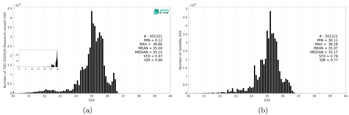
Figure 3: Histograms of SSS from TSG (GOSUD-Research-vessel) (a) and SMOS SSS L4 OI v346 - Weekly (CMEMS-CATDS-LOPS) (b) considering all match-up pairs per bins of 0.1 over the Tropical Pacific Ocean Pi-MEP region and for the full satellite product period.
