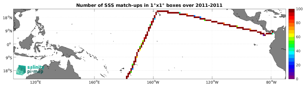
Figure 5: Number of SSS match-ups between TSG (CSIC-UTM) SSS and the SMOS SSS L4 OI v346 - Weekly (CMEMS-CATDS-LOPS) SSS product for the Tropical Pacific Ocean Pi-MEP region over 1^\circ \times 1^\circ boxes and for the full satellite product period.
