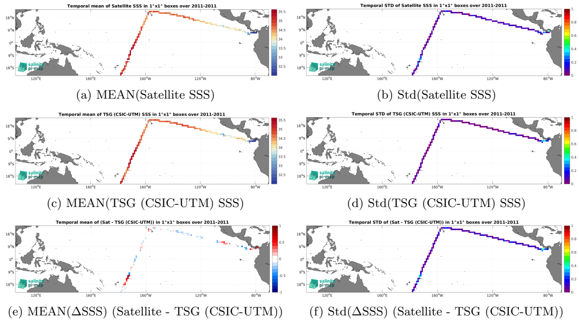
Figure 7: Temporal mean (left) and Std (right) of SSS from SMOS SSS L4 OI v346 - Weekly (CMEMS-CATDS-LOPS) (top), TSG (CSIC-UTM) (middle), and of \Delta SSS (Satellite - TSG (CSIC-UTM)). Only match-up pairs are used to generate these maps.
