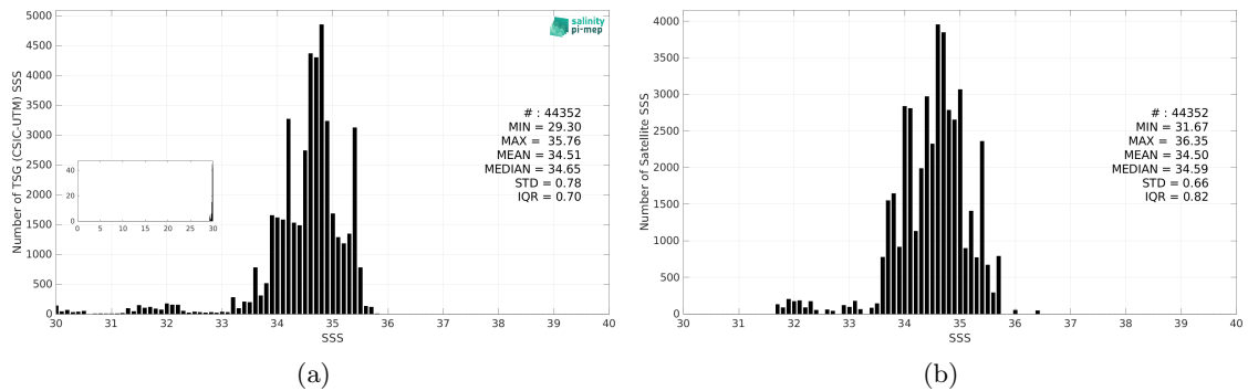
Figure 3: Histograms of SSS from TSG (CSIC-UTM) (a) and SMOS SSS L4 OI v346 - Weekly (CMEMS-CATDS-LOPS) (b) considering all match-up pairs per bins of 0.1 over the Tropical Pacific Ocean Pi-MEP region and for the full satellite product period.
