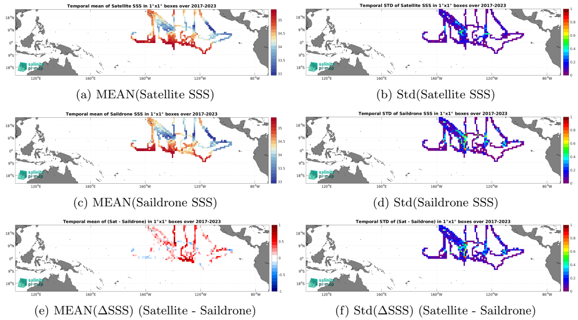
Figure 7: Temporal mean (left) and Std (right) of SSS from SMOS SSS L4 OI v346 - Weekly (CMEMS-CATDS-LOPS) (top), Saildrone (middle), and of \Delta SSS (Satellite - Saildrone). Only match-up pairs are used to generate these maps.
