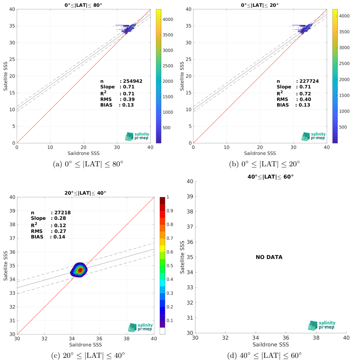
Figure 10: Contour maps of the concentration of SMOS SSS L4 OI v346 - Weekly (CMEMS-CATDS-LOPS) SSS (y-axis) versus Saildrone SSS (x-axis) at match-up pairs for different latitude bands. For each plot, the red line shows x=y . The black thin and dashed lines indicate a linear fit through the data cloud and the \pm 95\% confidence levels, respectively. The number match-up pairs n , the slope and R^2 coefficient of the linear fit, the root mean square (RMS) and the mean bias between satellite and in situ data are indicated for each latitude band in each plots.
