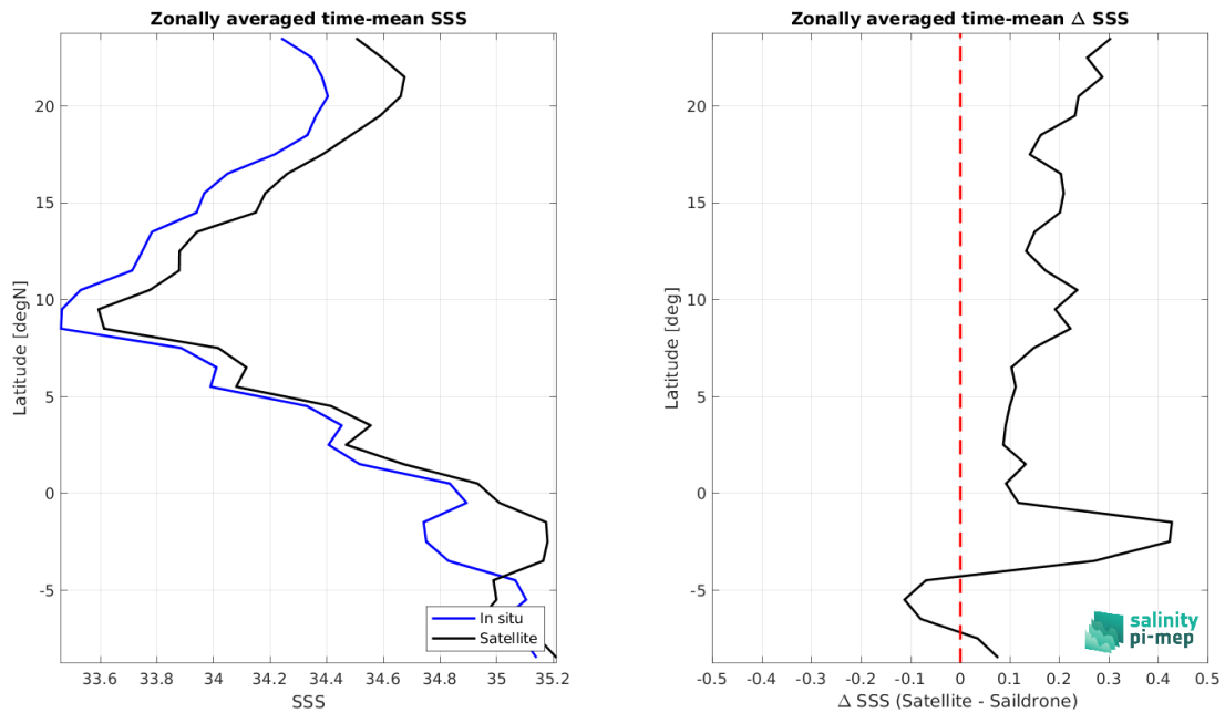
Figure 9: Left panel: Zonal mean SSS from SMOS SSS L4 OI v346 - Weekly (CMEMS-CATDS-LOPS) satellite product (black) and from Saildrone (blue). Right panel: Zonal mean of \Delta SSS (Satellite - Saildrone) for all the collected Pi-MEP match-up pairs estimated over the full satellite product period.
