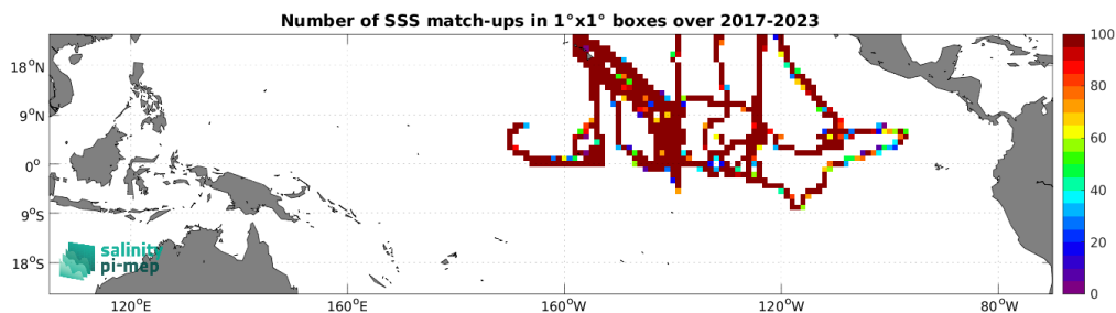
Figure 5: Number of SSS match-ups between Saildrone SSS and the SMOS SSS L4 OI v346 - Weekly (CMEMS-CATDS-LOPS) SSS product for the Tropical Pacific Ocean Pi-MEP region over 1^\circ \times 1^\circ boxes and for the full satellite product period.
