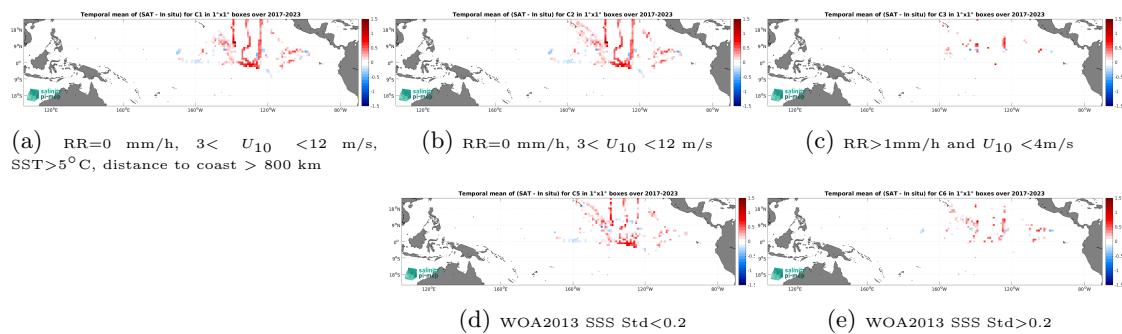
Figure 14: Temporal mean gridded over spatial boxes of size 1^\circ \times 1^\circ of \Delta SSS (SMOS SSS L4 OI v346 - Weekly (CMEMS-CATDS-LOPS) - Saildrone) for 5 different subdatasets corresponding to: RR=0 mm/h, 3 < U_{10} < 12 m/s, SST > 5°C, distance to coast > 800 km (a), RR=0 mm/h, 3 < U_{10} < 12 m/s (b), RR > 1mm/h and U_{10} < 4 m/s (c), WOA2013 SSS Std < 0.2 (d), WOA2013 SSS Std > 0.2 (e).
