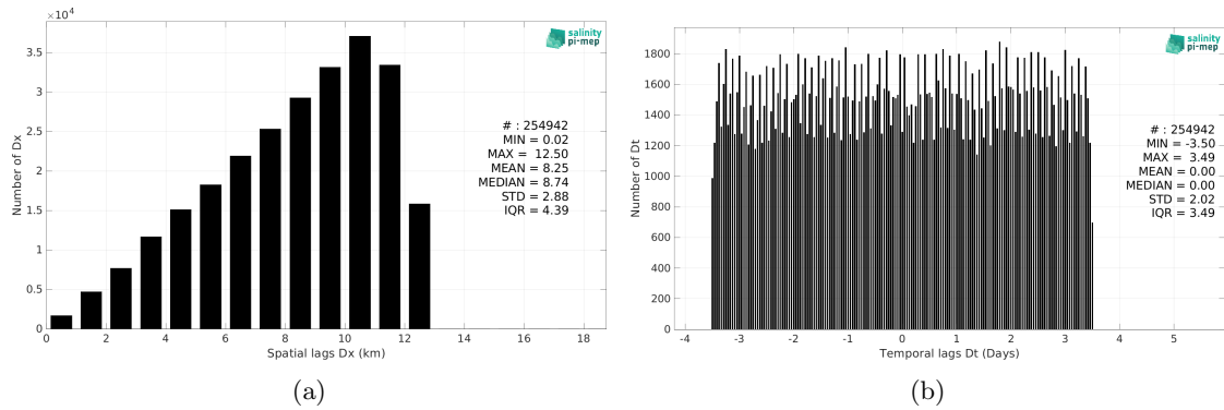
Figure 6: Histograms of the spatial (a) and temporal (b) lags between the location/time of the Sairdrone measurement and the date of the corresponding SMOS SSS L4 OI v346 - Weekly (CMEMS-CATDS-LOPS) SSS pixel.
