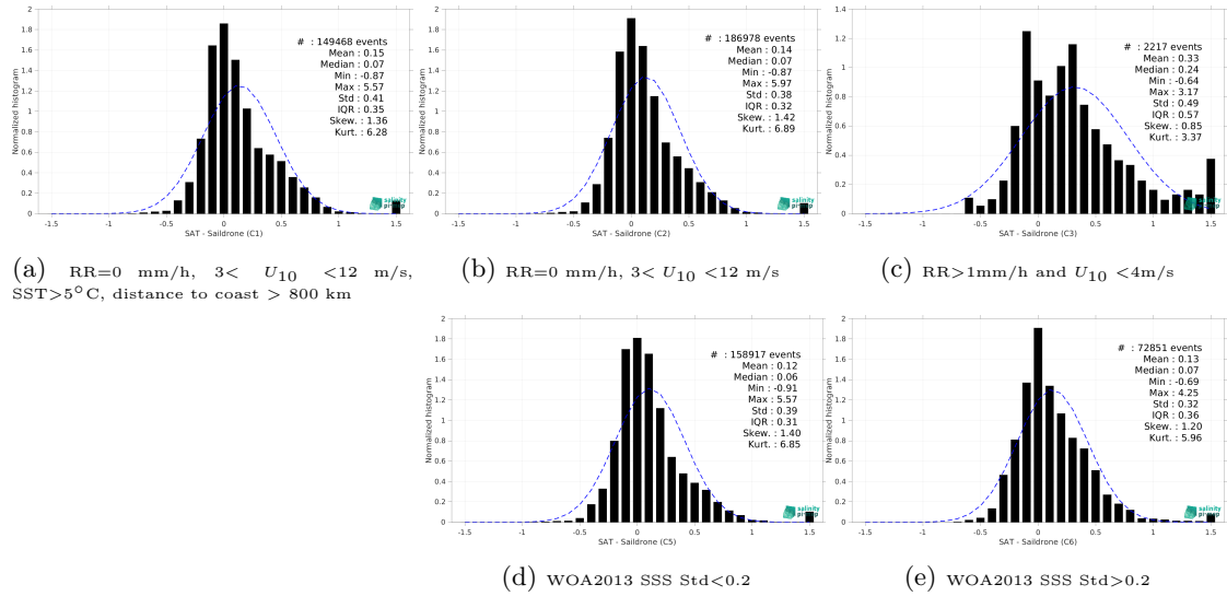
Figure 15: Normalized histogram of \Delta SSS (SMOS SSS L4 OI v346 - Weekly (CMEMS-CATDS-LOPS) - Saldrone) for 5 different subdatasets corresponding to: RR=0 mm/h, 3 < U_{10} < 12 m/s, SST>5°C, distance to coast > 800 km (a), RR=0 mm/h, 3 < U_{10} < 12 m/s (b), RR>1mm/h and U_{10} < 4 m/s (c), WOA2013 SSS Std<0.2 (d), WOA2013 SSS Std>0.2 (e).
