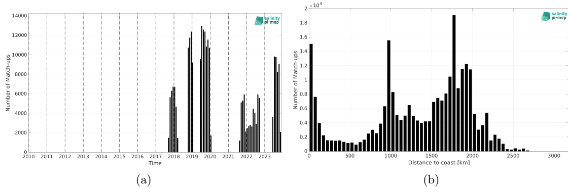
Figure 2: Number of match-ups between Saildrone and SMOS SSS L4 OI v346 - Weekly (CMEMS-CATDS-LOPS) SSS as a function of time (a) and as function of the distance to coast (b) over the Tropical Pacific Ocean Pi-MEP region and for the full satellite product period.
