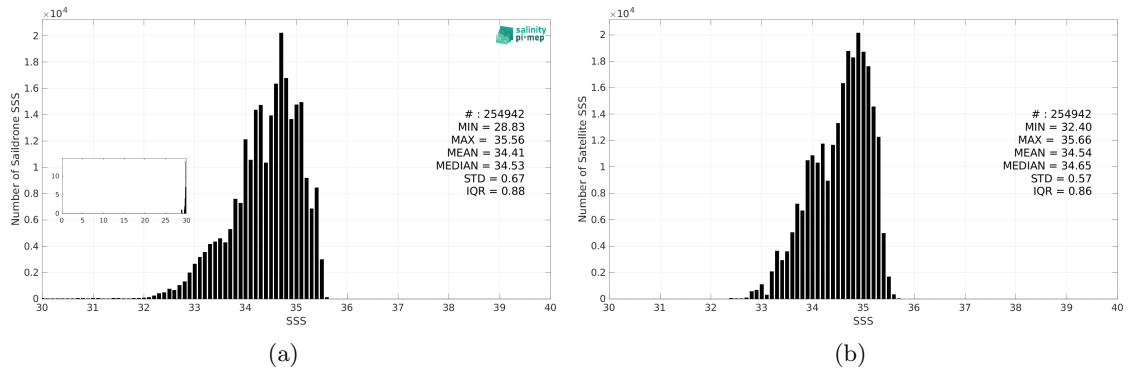
Figure 3: Histograms of SSS from Saildrone (a) and SMOS SSS L4 OI v346 - Weekly (CMEMS-CATDS-LOPS) (b) considering all match-up pairs per bins of 0.1 over the Tropical Pacific Ocean Pi-MEP region and for the full satellite product period.
