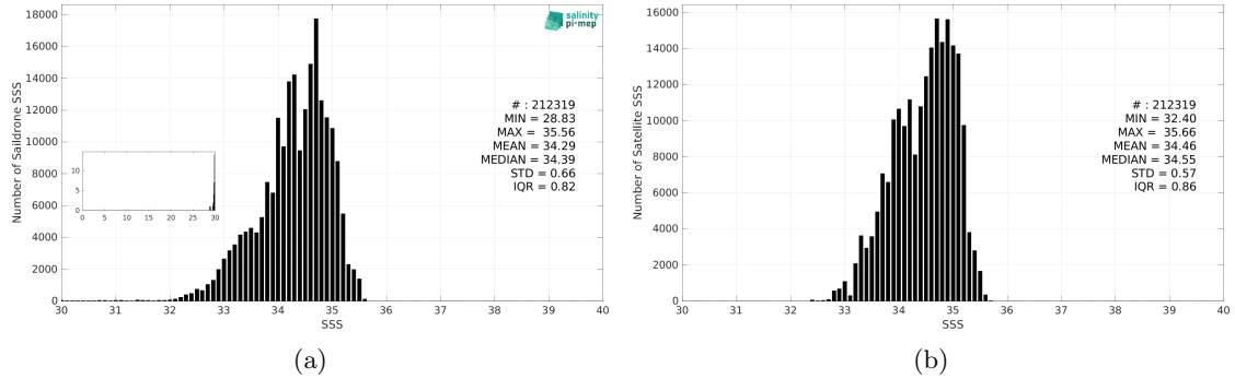
Figure 3: Histograms of SSS from Saildrone (a) and SMOS SSS L4 OI v346 - Weekly (CMEMS-CATDS-LOPS) (b) considering all match-up pairs per bins of 0.1 over the Tropical Pacific Ocean Pi-MEP region and for the full satellite product period.
