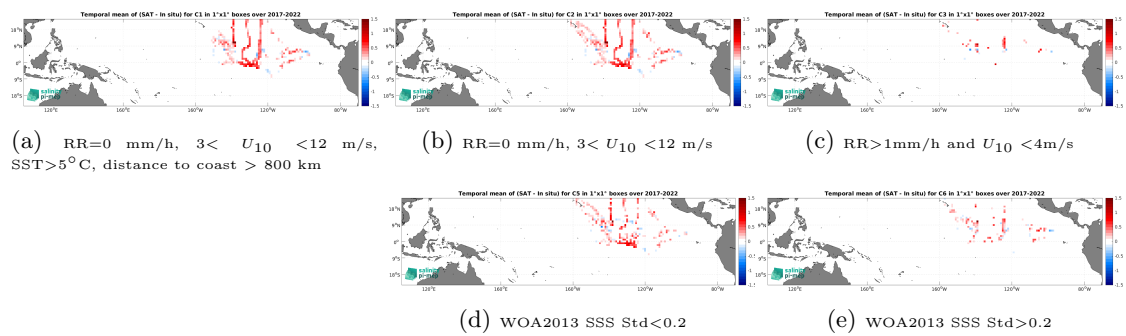
Figure 14: Temporal mean gridded over spatial boxes of size 1^\circ \times 1^\circ of \Delta\text{SSS} (SMOS SSS L4 OI v346 - Weekly (CMEMS-CATDS-LOPS) - Saildrone) for 5 different subdatasets corresponding to: RR=0 mm/h, 3 < U_{10} < 12 m/s, SST > 5°C, distance to coast > 800 km (a), RR=0 mm/h, 3 < U_{10} < 12 m/s (b), RR > 1mm/h and U_{10} < 4 m/s (c), WOA2013 SSS Std < 0.2 (d), WOA2013 SSS Std > 0.2 (e).
