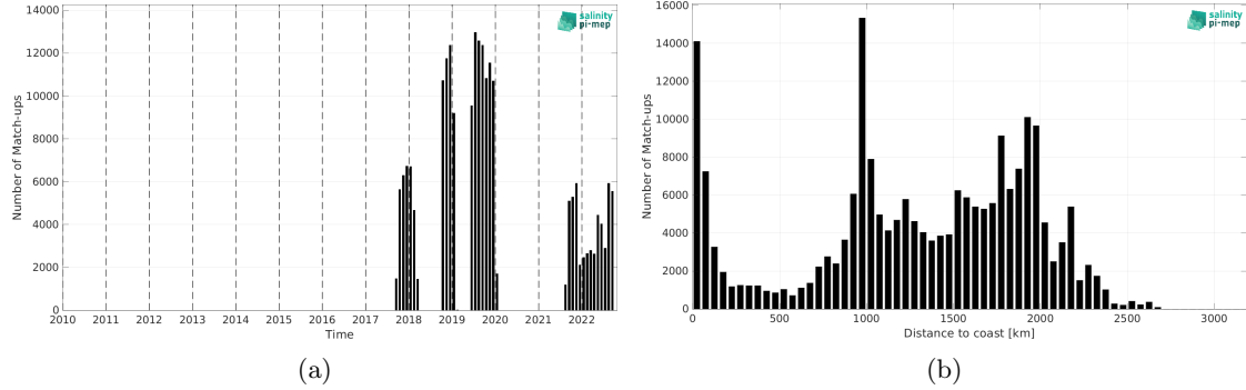
Figure 2: Number of match-ups between Saildrone and SMOS SSS L4 OI v346 - Weekly (CMEMS-CATDS-LOPS) SSS as a function of time (a) and as function of the distance to coast (b) over the Tropical Pacific Ocean Pi-MEP region and for the full satellite product period.
