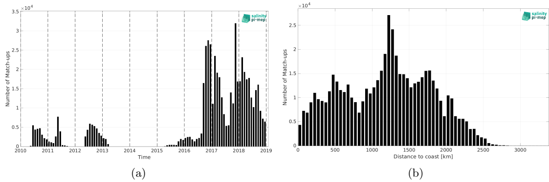
Figure 2: Number of match-ups between Surface drifters and SMOS SSS L4 OI v346 - Weekly (CMEMS-CATDS-LOPS) SSS as a function of time (a) and as function of the distance to coast (b) over the Tropical Pacific Ocean Pi-MEP region and for the full satellite product period.
