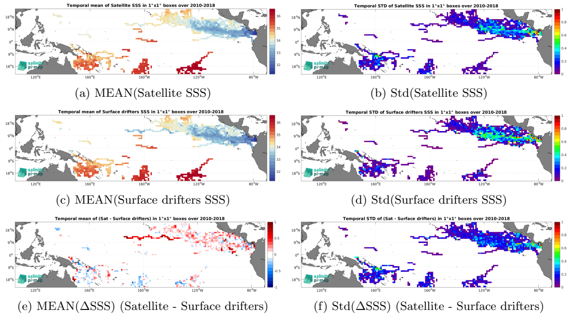
Figure 6: Temporal mean (left) and Std (right) of SSS from SMOS SSS L4 OI v346 - Weekly (CMEMS-CATDS-LOPS) (top), Surface drifters (middle), and of \Delta SSS (Satellite - Surface drifters). Only match-up pairs are used to generate these maps.
