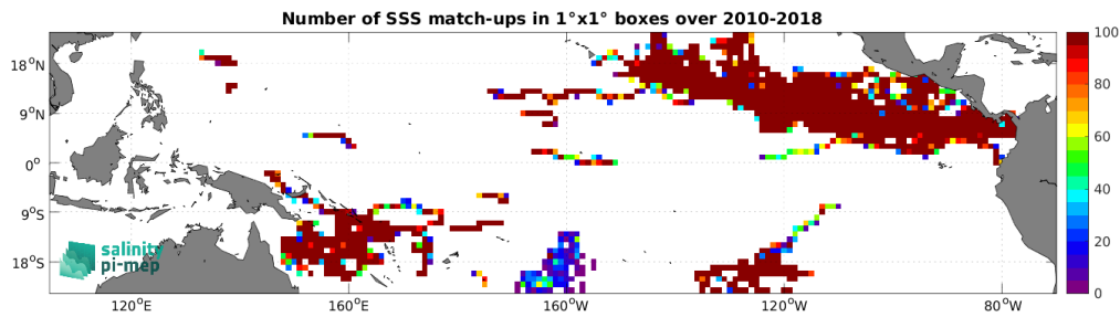
Figure 4: Number of SSS match-ups between Surface drifters SSS and the SMOS SSS L4 OI v346 - Weekly (CMEMS-CATDS-LOPS) SSS product for the Tropical Pacific Ocean Pi-MEP region over 1^\circ \times 1^\circ boxes and for the full satellite product period.
