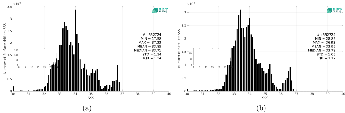
Figure 3: Histograms of SSS from Surface drifters (a) and SMOS SSS L4 OI v346 - Weekly (CMEMS-CATDS-LOPS) (b) considering all match-up pairs per bins of 0.1 over the Tropical Pacific Ocean Pi-MEP region and for the full satellite product period.
