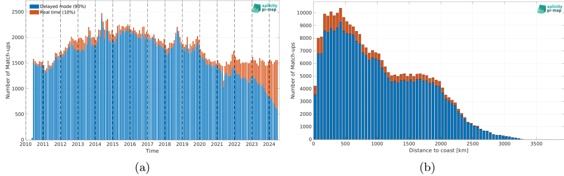
Figure 2: Number of match-ups between Argo and SMOS SSS L4 OI v346 - Weekly (CMEMS-CATDS-LOPS) SSS as a function of time (a) and as function of the distance to coast (b) over the Tropical Pacific Ocean Pi-MEP region and for the full satellite product period.
