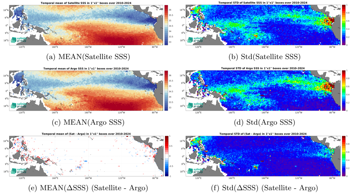
Figure 7: Temporal mean (left) and Std (right) of SSS from SMOS SSS L4 OI v346 - Weekly (CMEMS-CATDS-LOPS) (top), Argo (middle), and of \Delta SSS (Satellite - Argo). Only match-up pairs are used to generate these maps.
