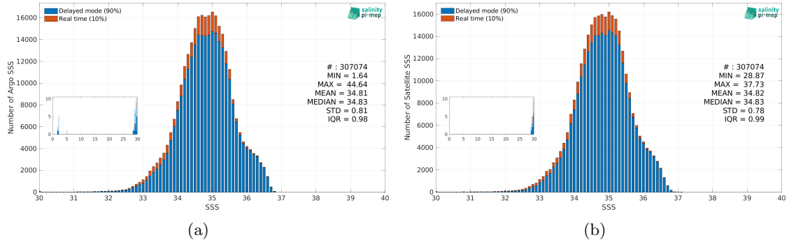
Figure 3: Histograms of SSS from Argo (a) and SMOS SSS L4 OI v346 - Weekly (CMEMS-CATDS-LOPS) (b) considering all match-up pairs per bins of 0.1 over the Tropical Pacific Ocean Pi-MEP region and for the full satellite product period.
