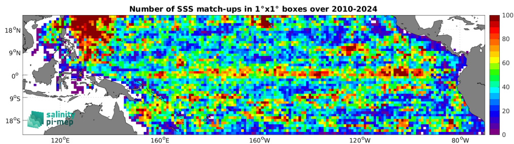
Figure 5: Number of SSS match-ups between Argo SSS and the SMOS SSS L4 OI v346 - Weekly (CMEMS-CATDS-LOPS) SSS product for the Tropical Pacific Ocean Pi-MEP region over 1^\circ \times 1^\circ boxes and for the full satellite product period.
