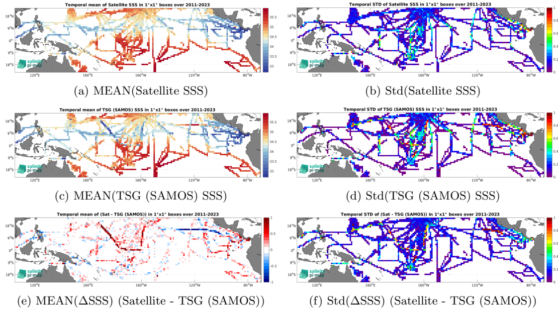
Figure 6: Temporal mean (left) and Std (right) of SSS from SMOS SSS L4 OI v342 - Weekly (CMEMS-CATDS-LOPS) (top), TSG (SAMOS) (middle), and of \Delta SSS (Satellite - TSG (SAMOS)). Only match-up pairs are used to generate these maps.
