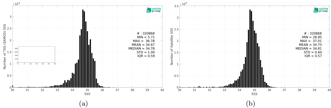
Figure 2: Histograms of SSS from TSG (SAMOS) (a) and SMOS SSS L4 OI v342 - Weekly (CMEMS-CATDS-LOPS) (b) considering all match-up pairs per bins of 0.1 over the Tropical Pacific Ocean Pi-MEP region and for the full satellite product period.
