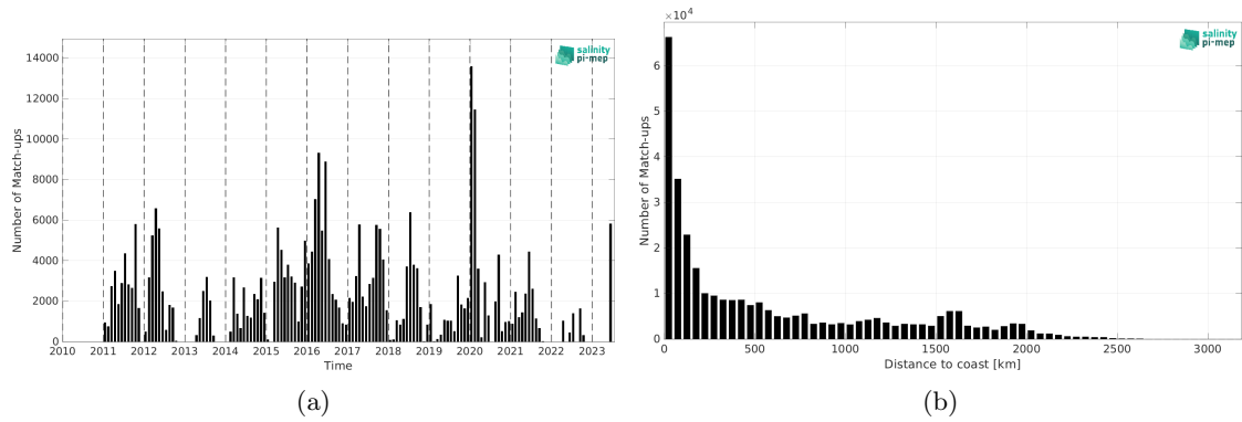
Figure 1: Number of match-ups between TSG (SAMOS) and SMOS SSS L4 OI v342 - Weekly (CMEMS-CATDS-LOPS) SSS as a function of time (a) and as function of the distance to coast (b) over the Tropical Pacific Ocean Pi-MEP region and for the full satellite product period.
