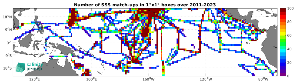
Figure 4: Number of SSS match-ups between TSG (SAMOS) SSS and the SMOS SSS L4 OI v342 - Weekly (CMEMS-CATDS-LOPS) SSS product for the Tropical Pacific Ocean Pi-MEP region over 1^\circ \times 1^\circ boxes and for the full satellite product period.
