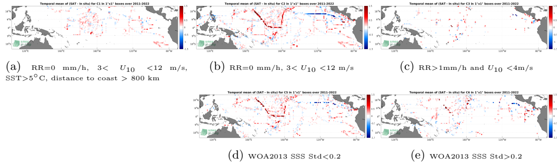
Figure 12: Temporal mean gridded over spatial boxes of size 1^{\circ}\times 1^{\circ} of \Delta\text{SSS} (SMOS SSS L4 OI v342 - Weekly (CMEMS-CATDS-LOPS) - TSG (SAMOS)) for 5 different subdatasets corresponding to:RR=0 mm/h, 3 < U_{10} < 12 m/s, SST >5^{\circ}\text{C} , distance to coast > 800 km (a), RR=0 mm/h, 3 < U_{10} < 12 m/s (b), RR >1 mm/h and U_{10} < 4 m/s (c), WOA2013 SSS Std <0.2 (d), WOA2013 SSS Std >0.2 (e).
