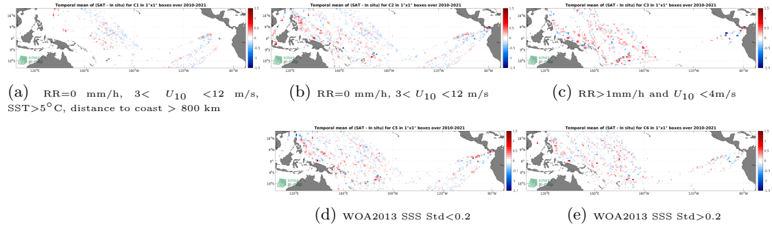
Figure 12: Temporal mean gridded over spatial boxes of size 1^{\circ}\times 1^{\circ} of \Delta\text{SSS} (SMOS SSS L4 OI v342 - Weekly (CMEMS-CATDS-LOPS) - TSG (LEGOS-DM)) for 5 different subdatasets corresponding to:RR=0 mm/h, 3 < U_{10} < 12 m/s, SST >5^{\circ}\text{C} , distance to coast > 800 km (a), RR=0 mm/h, 3 < U_{10} < 12 m/s (b), RR >1 mm/h and U_{10} < 4 m/s (c), WOA2013 SSS Std <0.2 (d), WOA2013 SSS Std >0.2 (e).
