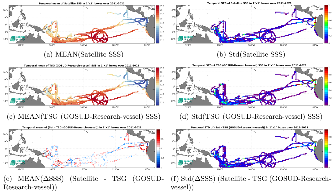
Figure 6: Temporal mean (left) and Std (right) of SSS from SMOS SSS L4 OI v342 - Weekly (CMEMS-CATDS-LOPS) (top), TSG (GOSUD-Research-vessel) (middle), and of \Delta SSS (Satellite - TSG (GOSUD-Research-vessel)). Only match-up pairs are used to generate these maps.
