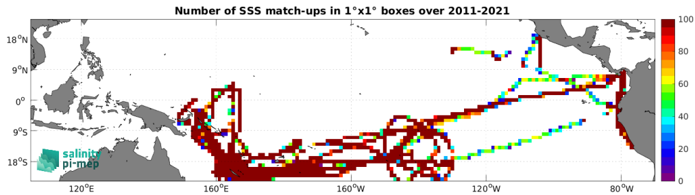
Figure 4: Number of SSS match-ups between TSG (GOSUD-Research-vessel) SSS and the SMOS SSS L4 OI v342 - Weekly (CMEMS-CATDS-LOPS) SSS product for the Tropical Pacific Ocean Pi-MEP region over 1°x1° boxes and for the full satellite product period.
