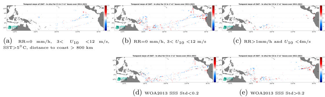
Figure 12: Temporal mean gridded over spatial boxes of size 1^\circ \times 1^\circ of \Delta SSS (SMOS SSS L4 OI v342 - Weekly (CMEMS-CATDS-LOPS) - TSG (GOSUD-Research-vessel)) for 5 different subdatasets corresponding to:RR=0 mm/h, 3 < U_{10} < 12 m/s, SST > 5^\circ\text{C} , distance to coast > 800 km (a), RR=0 mm/h, 3 < U_{10} < 12 m/s (b), RR > 1 mm/h and U_{10} < 4 m/s (c), WOA2013 SSS Std < 0.2 (d), WOA2013 SSS Std > 0.2 (e).
