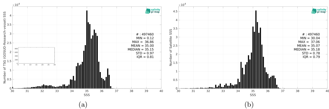
Figure 2: Histograms of SSS from TSG (GOSUD-Research-vessel) (a) and SMOS SSS L4 OI v342 - Weekly (CMEMS-CATDS-LOPS) (b) considering all match-up pairs per bins of 0.1 over the Tropical Pacific Ocean Pi-MEP region and for the full satellite product period.
