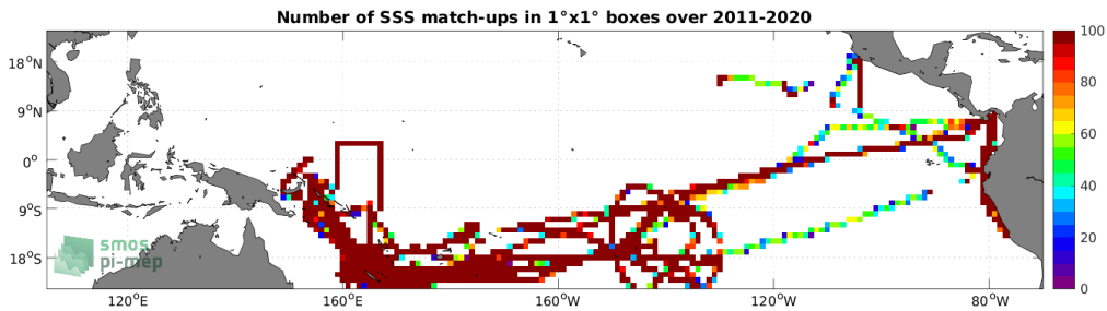
Figure 4: Number of SSS match-ups between TSG (GOSUD-Research-vessel) SSS and the SMOS SSS L4 OI v342 - Weekly (CMEMS-CATDS-LOPS) SSS product for the Tropical Pacific Ocean Pi-MEP region over 1^\circ \times 1^\circ boxes and for the full satellite product period.
