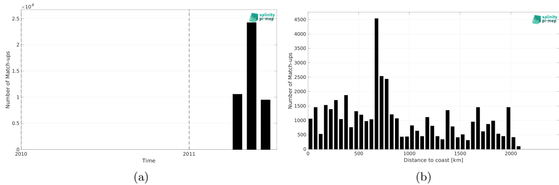
Figure 1: Number of match-ups between TSG (CSIC-UTM) and SMOS SSS L4 OI v342 - Weekly (CMEMS-CATDS-LOPS) SSS as a function of time (a) and as function of the distance to coast (b) over the Tropical Pacific Ocean Pi-MEP region and for the full satellite product period.
