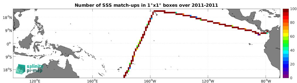
Figure 4: Number of SSS match-ups between TSG (CSIC-UTM) SSS and the SMOS SSS L4 OI v342 - Weekly (CMEMS-CATDS-LOPS) SSS product for the Tropical Pacific Ocean Pi-MEP region over 1^\circ \times 1^\circ boxes and for the full satellite product period.
