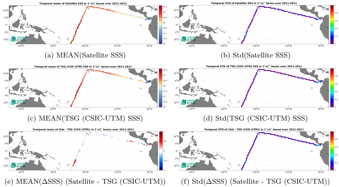
Figure 6: Temporal mean (left) and Std (right) of SSS from SMOS SSS L4 OI v342 - Weekly (CMEMS-CATDS-LOPS) (top), TSG (CSIC-UTM) (middle), and of \Delta SSS (Satellite - TSG (CSIC-UTM)). Only match-up pairs are used to generate these maps.
