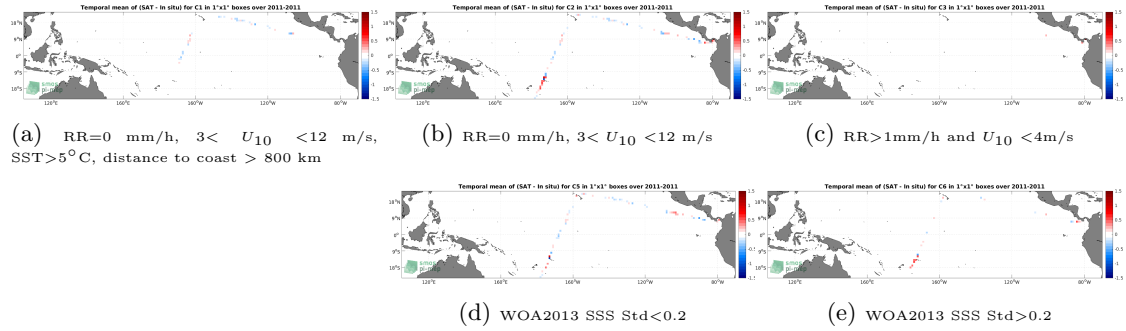
Figure 12: Temporal mean gridded over spatial boxes of size 1^{\circ}\times 1^{\circ} of \Delta\text{SSS} (SMOS SSS L4 OI v342 - Weekly (CMEMS-CATDS-LOPS) - TSG (CSIC-UTM)) for 5 different subdatasets corresponding to:RR=0 mm/h, 3 < U_{10} < 12 m/s, SST >5^{\circ}\text{C} , distance to coast > 800 km (a), RR=0 mm/h, 3 < U_{10} < 12 m/s (b), RR >1 mm/h and U_{10} < 4 m/s (c), WOA2013 SSS Std <0.2 (d), WOA2013 SSS Std >0.2 (e).
