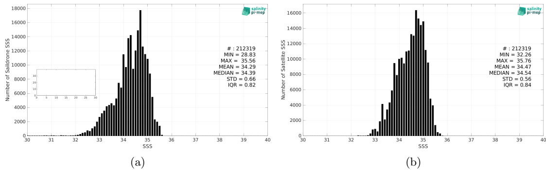
Figure 2: Histograms of SSS from Saildrone (a) and SMOS SSS L4 OI v342 - Weekly (CMEMS-CATDS-LOPS) (b) considering all match-up pairs per bins of 0.1 over the Tropical Pacific Ocean Pi-MEP region and for the full satellite product period.
