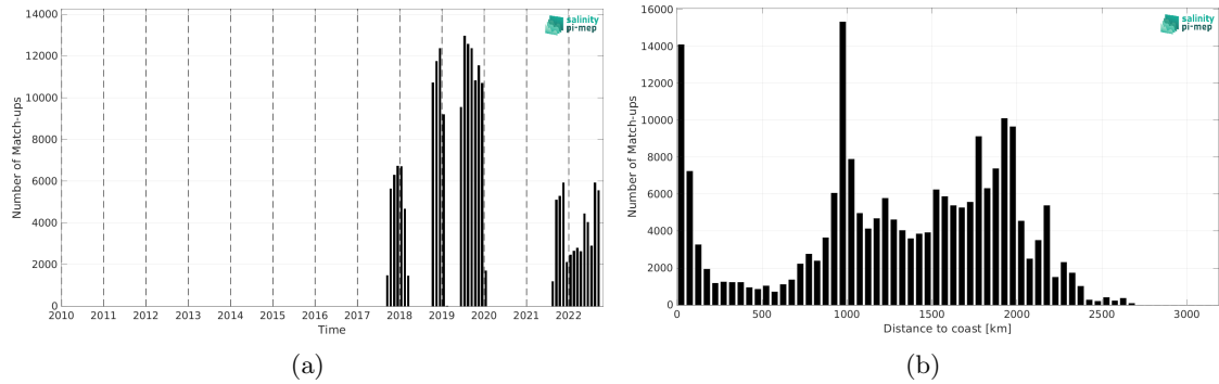
Figure 1: Number of match-ups between Saildrone and SMOS SSS L4 OI v342 - Weekly (CMEMS-CATDS-LOPS) SSS as a function of time (a) and as function of the distance to coast (b) over the Tropical Pacific Ocean Pi-MEP region and for the full satellite product period.
