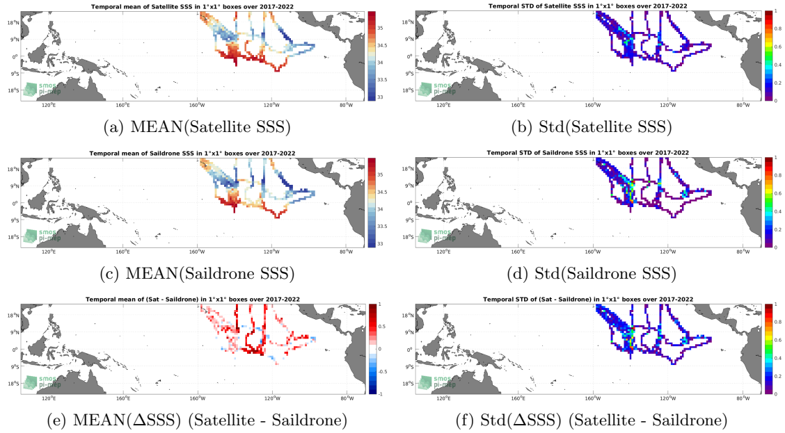
Figure 6: Temporal mean (left) and Std (right) of SSS from SMOS SSS L4 OI v342 - Weekly (CMEMS-CATDS-LOPS) (top), Saildrone (middle), and of \Delta SSS (Satellite - Saildrone). Only match-up pairs are used to generate these maps.
