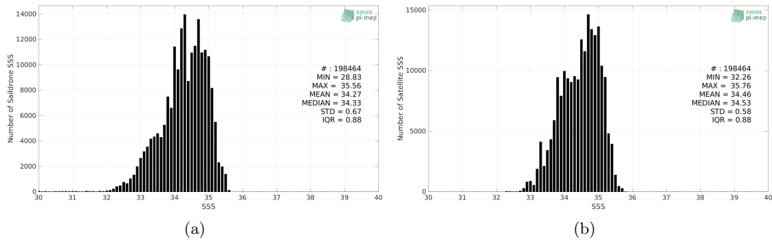
Figure 2: Histograms of SSS from Sairdrone (a) and SMOS SSS L4 OI v342 - Weekly (CMEMS-CATDS-LOPS) (b) considering all match-up pairs per bins of 0.1 over the Tropical Pacific Ocean Pi-MEP region and for the full satellite product period.
