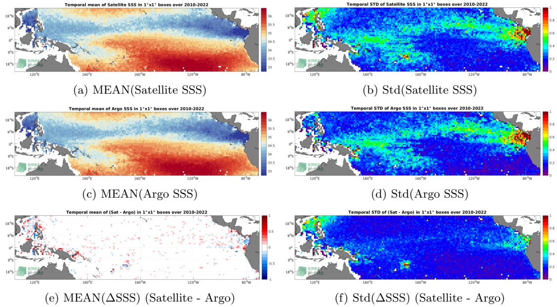
Figure 6: Temporal mean (left) and Std (right) of SSS from SMOS SSS L4 OI v342 - Weekly (CMEMS-CATDS-LOPS) (top), Argo (middle), and of \Delta SSS (Satellite - Argo). Only match-up pairs are used to generate these maps.
