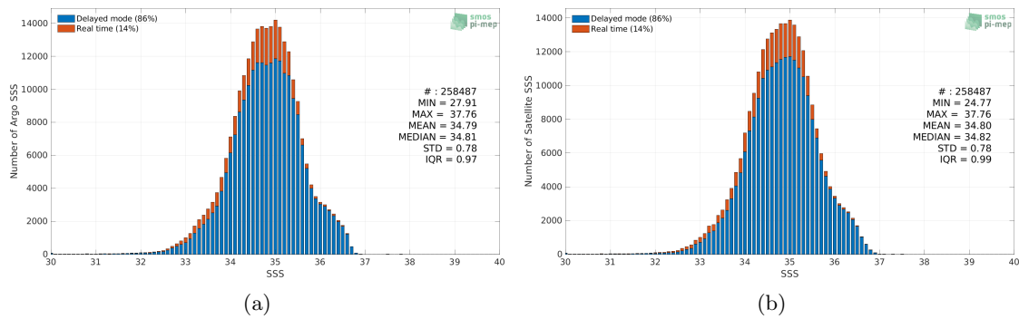
Figure 2: Histograms of SSS from Argo (a) and SMOS SSS L4 OI v342 - Weekly (CMEMS-CATDS-LOPS) (b) considering all match-up pairs per bins of 0.1 over the Tropical Pacific Ocean Pi-MEP region and for the full satellite product period.
