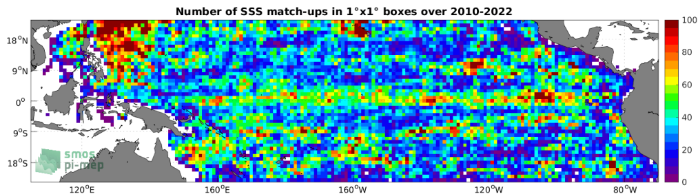
Figure 4: Number of SSS match-ups between Argo SSS and the SMOS SSS L4 OI v342 - Weekly (CMEMS-CATDS-LOPS) SSS product for the Tropical Pacific Ocean Pi-MEP region over 1^\circ \times 1^\circ boxes and for the full satellite product period.
