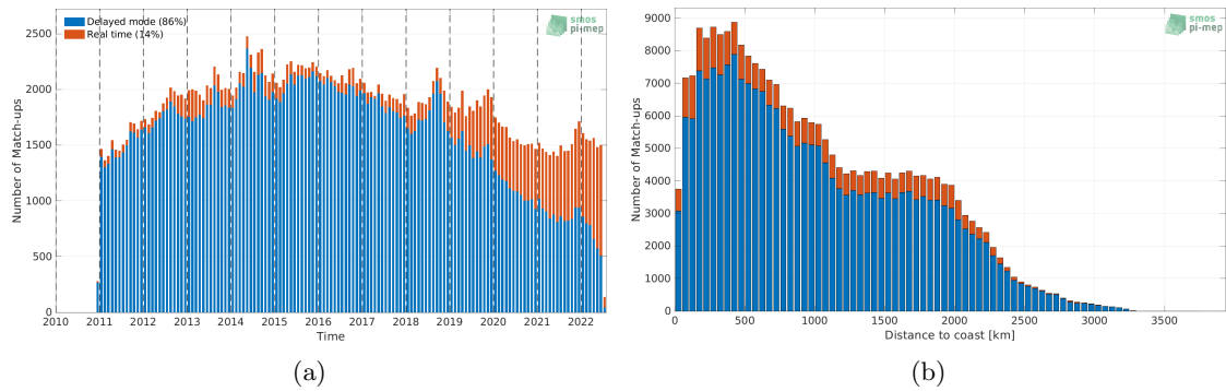
Figure 1: Number of match-ups between Argo and SMOS SSS L4 OI v342 - Weekly (CMEMS-CATDS-LOPS) SSS as a function of time (a) and as function of the distance to coast (b) over the Tropical Pacific Ocean Pi-MEP region and for the full satellite product period.
