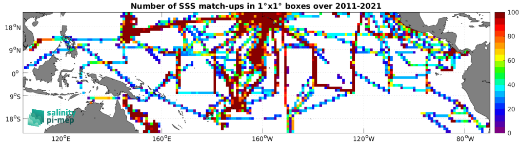
Figure 4: Number of SSS match-ups between TSG (SAMOS) SSS and the SMOS SSS L4 v2 - Daily (BEC) SSS product for the Tropical Pacific Ocean Pi-MEP region over 1^\circ \times 1^\circ boxes and for the full satellite product period.
