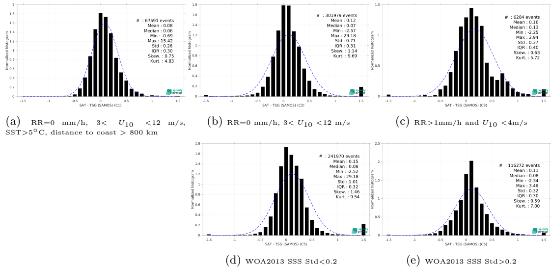
Figure 13: Normalized histogram of \Delta\text{SSS} (SMOS SSS L4 v2 - Daily (BEC) - TSG (SAMOS)) for 5 different subdatasets corresponding to: RR=0 mm/h, 3 < U_{10} < 12 m/s, SST >5^\circ\text{C} , distance to coast > 800 km (a), RR=0 mm/h, 3 < U_{10} < 12 m/s (b), RR >1 mm/h and U_{10} < 4 m/s (c), WOA2013 SSS Std <0.2 (d), WOA2013 SSS Std >0.2 (e).
