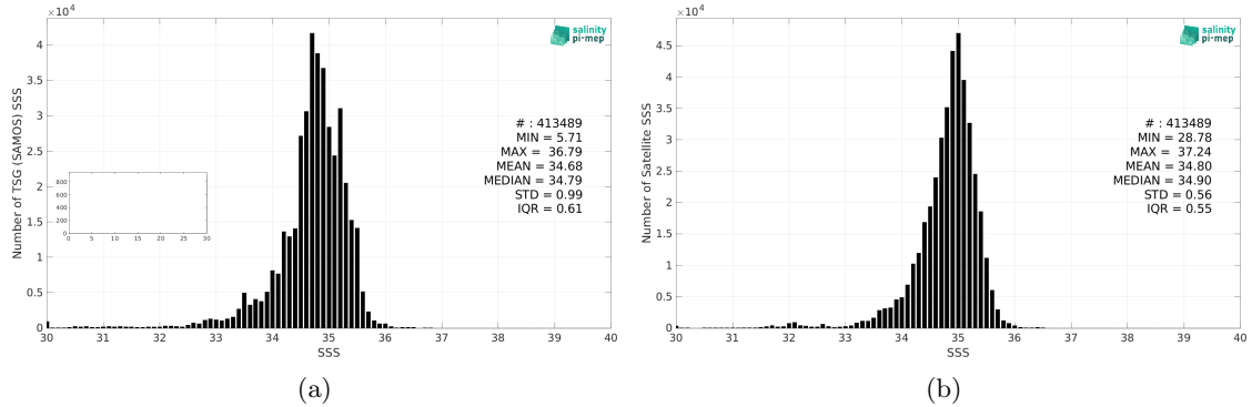
Figure 2: Histograms of SSS from TSG (SAMOS) (a) and SMOS SSS L4 v2 - Daily (BEC) (b) considering all match-up pairs per bins of 0.1 over the Tropical Pacific Ocean Pi-MEP region and for the full satellite product period.
