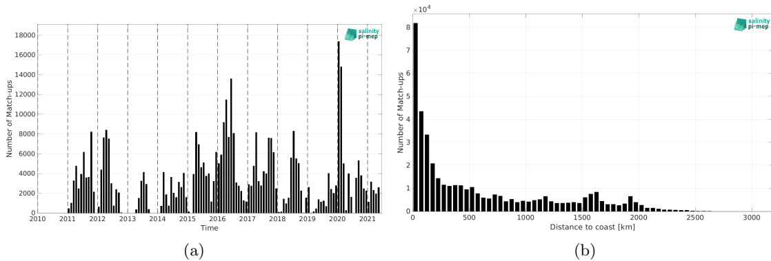
Figure 1: Number of match-ups between TSG (SAMOS) and SMOS SSS L4 v2 - Daily (BEC) SSS as a function of time (a) and as function of the distance to coast (b) over the Tropical Pacific Ocean Pi-MEP region and for the full satellite product period.
