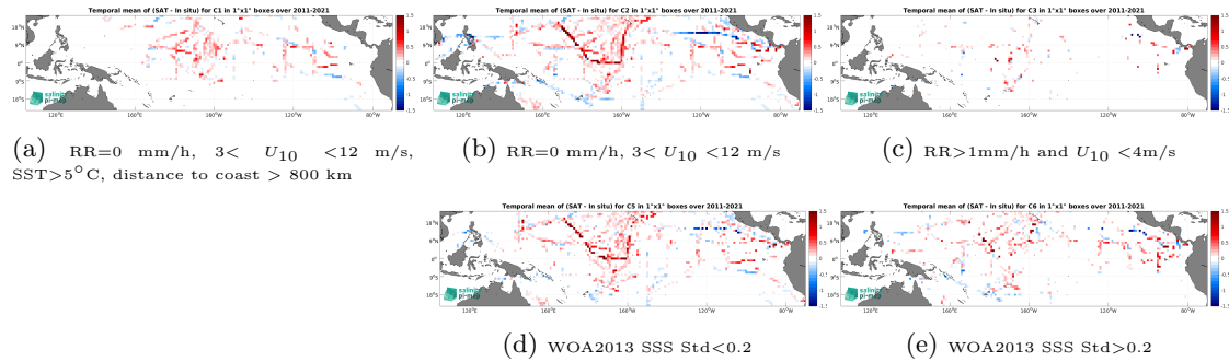
Figure 12: Temporal mean gridded over spatial boxes of size 1^\circ \times 1^\circ of \Delta\text{SSS} (SMOS SSS L4 v2 - Daily (BEC) - TSG (SAMOS)) for 5 different subdatasets corresponding to:RR=0 mm/h, 3 < U_{10} < 12 m/s, SST >5^\circ\text{C} , distance to coast > 800 km (a), RR=0 mm/h, 3 < U_{10} < 12 m/s (b), RR >1 mm/h and U_{10} < 4 m/s (c), WOA2013 SSS Std <0.2 (d), WOA2013 SSS Std >0.2 (e).
