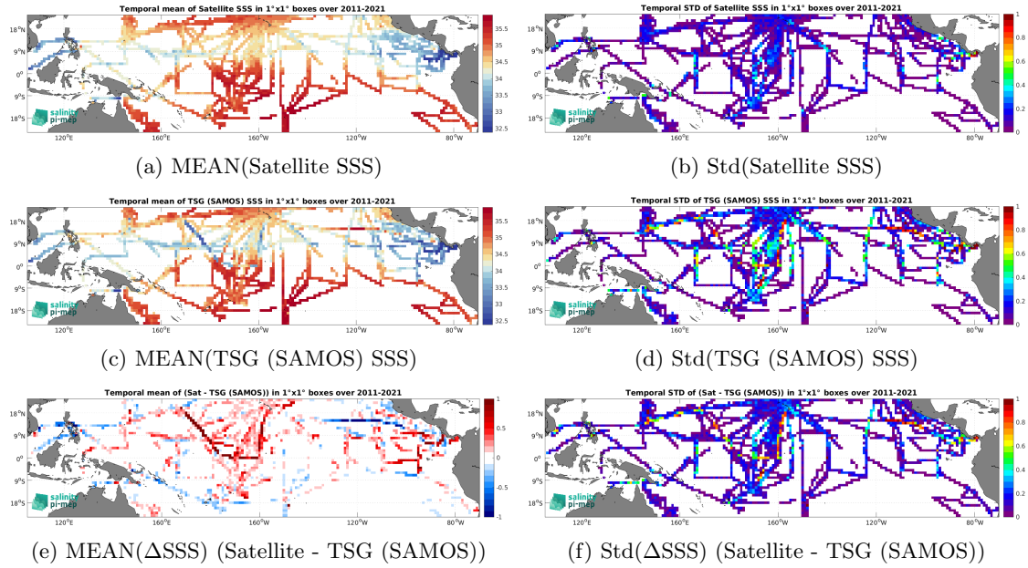
Figure 6: Temporal mean (left) and Std (right) of SSS from SMOS SSS L4 v2 - Daily (BEC) (top), TSG (SAMOS) (middle), and of \Delta SSS (Satellite - TSG (SAMOS)). Only match-up pairs are used to generate these maps.
