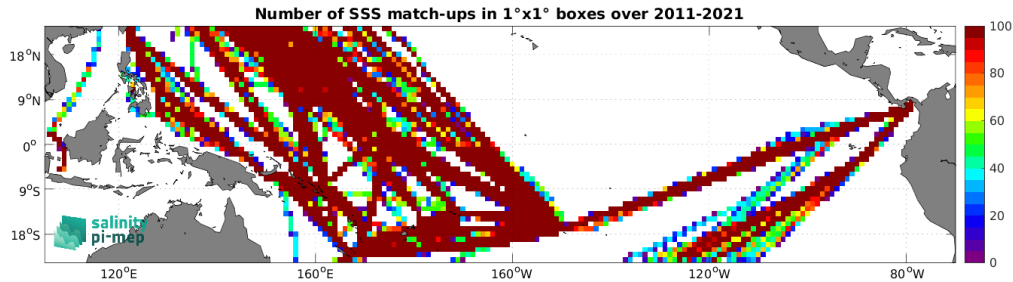
Figure 5: Number of SSS match-ups between TSG (LEGOS-DM) SSS and the SMOS SSS L4 v2 - Daily (BEC) SSS product for the Tropical Pacific Ocean Pi-MEP region over 1^\circ \times 1^\circ boxes and for the full satellite product period.
