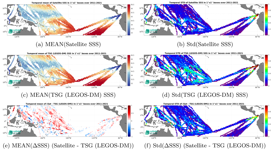
Figure 7: Temporal mean (left) and Std (right) of SSS from SMOS SSS L4 v2 - Daily (BEC) (top), TSG (LEGOS-DM) (middle), and of \Delta SSS (Satellite - TSG (LEGOS-DM)). Only match-up pairs are used to generate these maps.
