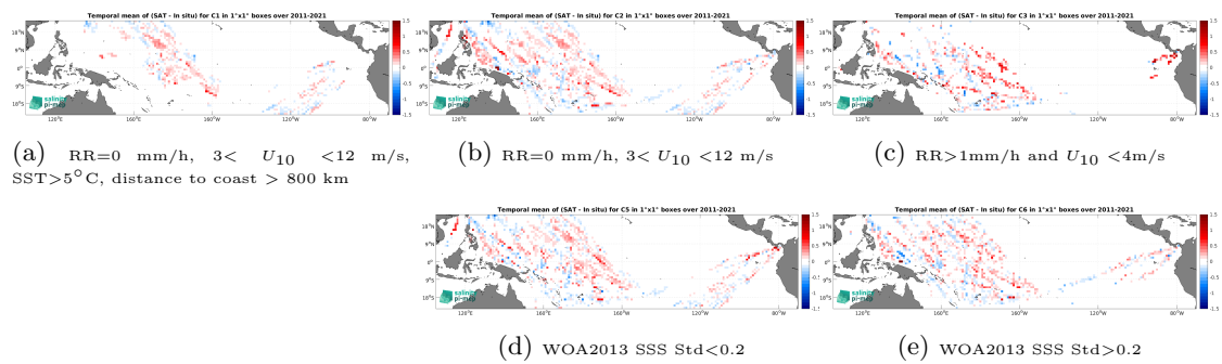
Figure 14: Temporal mean gridded over spatial boxes of size 1^\circ \times 1^\circ of \Delta SSS (SMOS SSS L4 v2 - Daily (BEC) - TSG (LEGOS-DM)) for 5 different subdatasets corresponding to: RR=0 mm/h, 3 < U_{10} < 12 m/s, SST > 5^\circ\text{C} , distance to coast > 800 km (a), RR=0 mm/h, 3 < U_{10} < 12 m/s (b), RR > 1 mm/h and U_{10} < 4 m/s (c), WOA2013 SSS Std < 0.2 (d), WOA2013 SSS Std > 0.2 (e).
