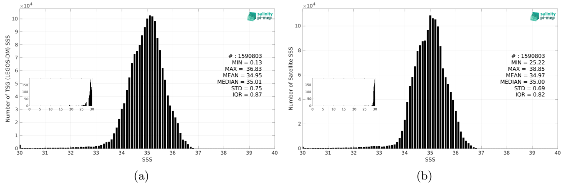
Figure 3: Histograms of SSS from TSG (LEGOS-DM) (a) and SMOS SSS L4 v2 - Daily (BEC) (b) considering all match-up pairs per bins of 0.1 over the Tropical Pacific Ocean Pi-MEP region and for the full satellite product period.
