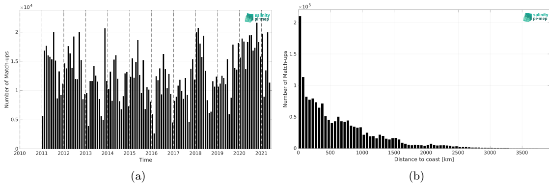
Figure 2: Number of match-ups between TSG (LEGOS-DM) and SMOS SSS L4 v2 - Daily (BEC) SSS as a function of time (a) and as function of the distance to coast (b) over the Tropical Pacific Ocean Pi-MEP region and for the full satellite product period.
