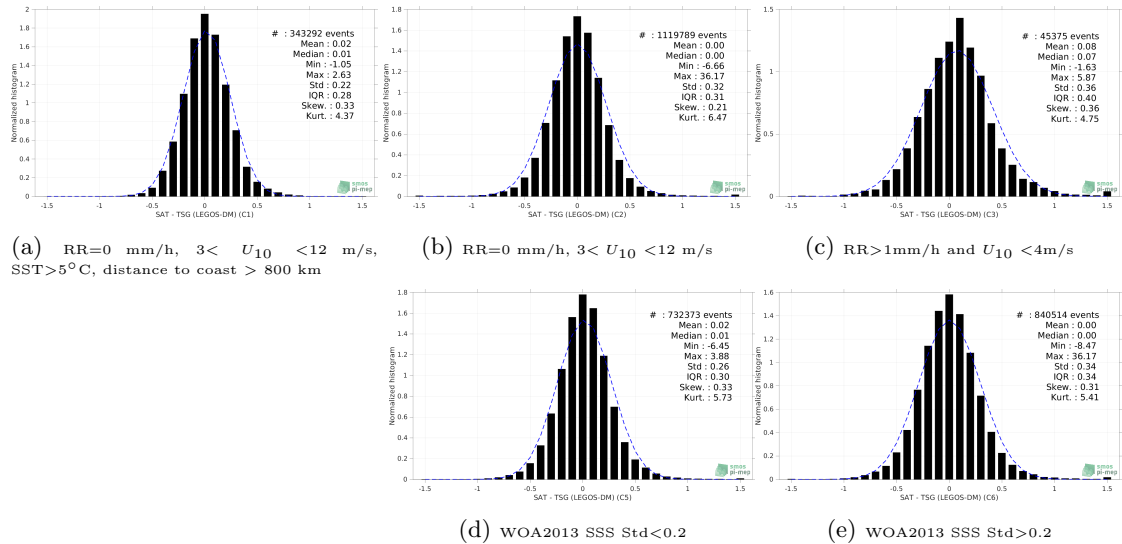
Figure 13: Normalized histogram of \Delta SSS (SMOS SSS L4 v2 - Daily (BEC) - TSG (LEGOS-DM)) for 5 different subdatasets corresponding to: RR=0 mm/h, 3 < U_{10} < 12 m/s, SST >5^\circ\text{C} , distance to coast > 800 km (a), RR=0 mm/h, 3 < U_{10} < 12 m/s (b), RR >1 mm/h and U_{10} < 4 m/s (c), WOA2013 SSS Std <0.2 (d), WOA2013 SSS Std >0.2 (e).
