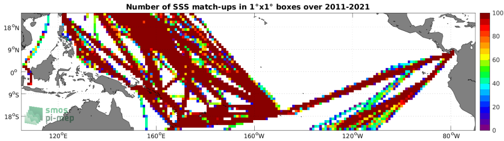
Figure 4: Number of SSS match-ups between TSG (LEGOS-DM) SSS and the SMOS SSS L4 v2 - Daily (BEC) SSS product for the Tropical Pacific Ocean Pi-MEP region over 1^\circ \times 1^\circ boxes and for the full satellite product period.
