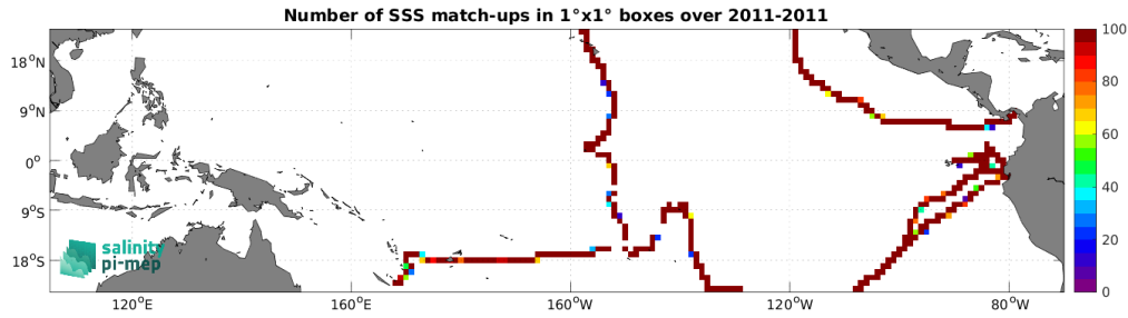
Figure 5: Number of SSS match-ups between TSG (GOSUD-Sailing-ship) SSS and the SMOS SSS L4 v2 - Daily (BEC) SSS product for the Tropical Pacific Ocean Pi-MEP region over 1^\circ \times 1^\circ boxes and for the full satellite product period.
