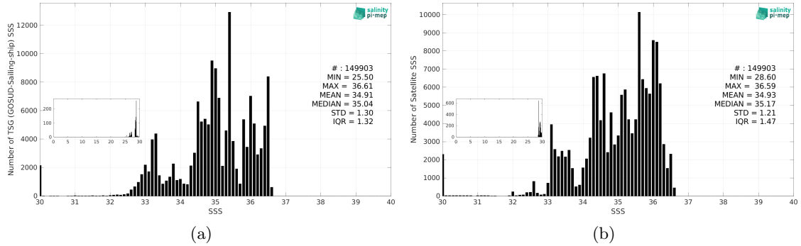
Figure 3: Histograms of SSS from TSG (GOSUD-Sailing-ship) (a) and SMOS SSS L4 v2 - Daily (BEC) (b) considering all match-up pairs per bins of 0.1 over the Tropical Pacific Ocean Pi-MEP region and for the full satellite product period.
