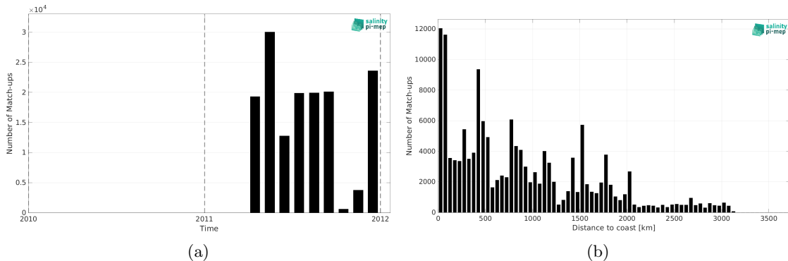
Figure 2: Number of match-ups between TSG (GOSUD-Sailing-ship) and SMOS SSS L4 v2 - Daily (BEC) SSS as a function of time (a) and as function of the distance to coast (b) over the Tropical Pacific Ocean Pi-MEP region and for the full satellite product period.
