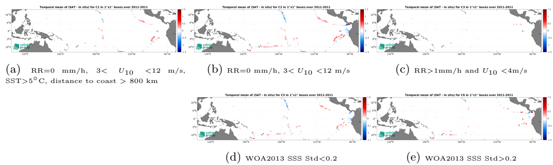
Figure 14: Temporal mean gridded over spatial boxes of size 1^\circ \times 1^\circ of \Delta SSS (SMOS SSS L4 v2 - Daily (BEC) - TSG (GOSUD-Sailing-ship)) for 5 different subdatasets corresponding to:RR=0 mm/h, 3 < U_{10} < 12 m/s, SST > 5^\circ\text{C} , distance to coast > 800 km (a), RR=0 mm/h, 3 < U_{10} < 12 m/s (b), RR > 1 mm/h and U_{10} < 4 m/s (c), WOA2013 SSS Std < 0.2 (d), WOA2013 SSS Std > 0.2 (e).
