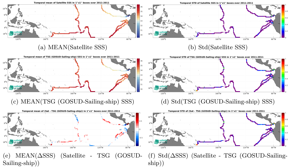
Figure 6: Temporal mean (left) and Std (right) of SSS from SMOS SSS L4 v2 - Daily (BEC) (top), TSG (GOSUD-Sailing-ship) (middle), and of \Delta SSS (Satellite - TSG (GOSUD-Sailing-ship)). Only match-up pairs are used to generate these maps.
