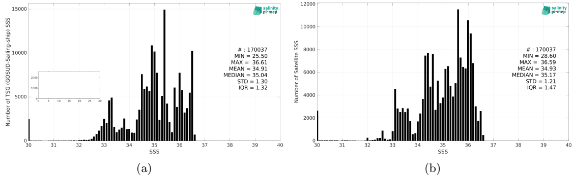
Figure 2: Histograms of SSS from TSG (GOSUD-Sailing-ship) (a) and SMOS SSS L4 v2 - Daily (BEC) (b) considering all match-up pairs per bins of 0.1 over the Tropical Pacific Ocean Pi-MEP region and for the full satellite product period.
