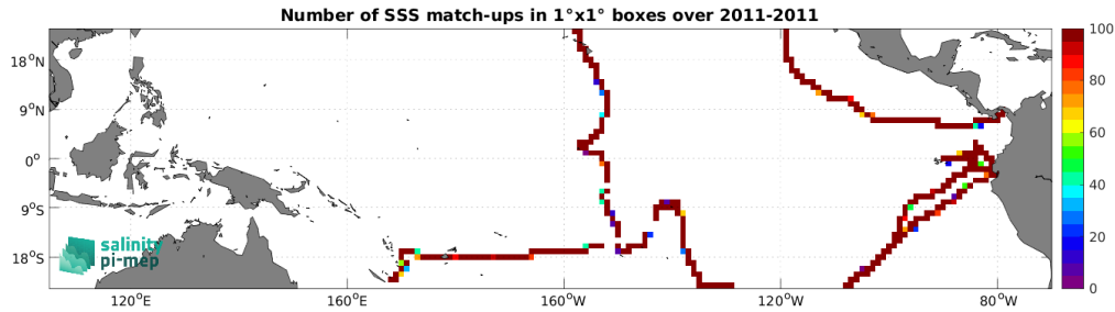
Figure 4: Number of SSS match-ups between TSG (GOSUD-Sailing-ship) SSS and the SMOS SSS L4 v2 - Daily (BEC) SSS product for the Tropical Pacific Ocean Pi-MEP region over 1^\circ \times 1^\circ boxes and for the full satellite product period.
