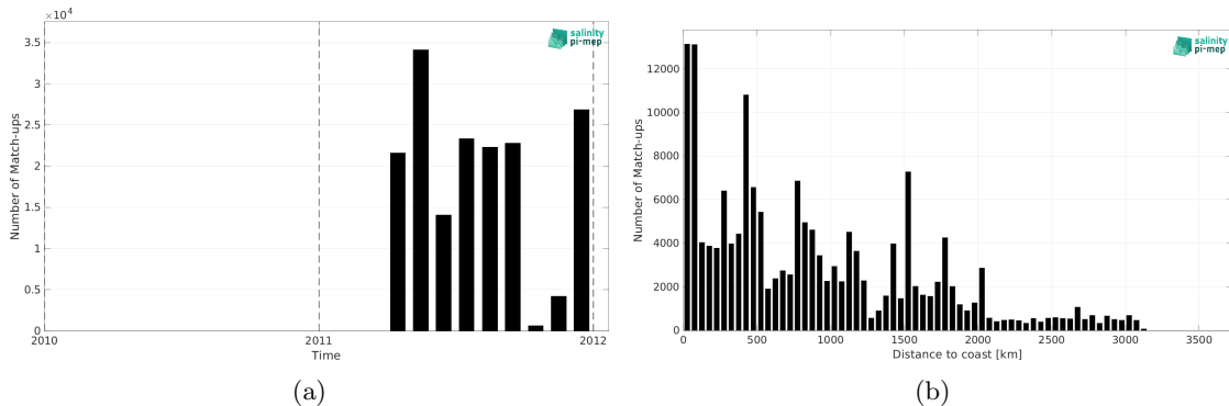
Figure 1: Number of match-ups between TSG (GOSUD-Sailing-ship) and SMOS SSS L4 v2 - Daily (BEC) SSS as a function of time (a) and as function of the distance to coast (b) over the Tropical Pacific Ocean Pi-MEP region and for the full satellite product period.
