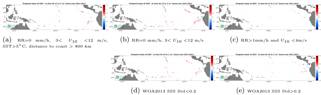
Figure 12: Temporal mean gridded over spatial boxes of size 1^\circ \times 1^\circ of \Delta SSS (SMOS SSS L4 v2 - Daily (BEC) - TSG (GOSUD-Sailing-ship)) for 5 different subdatasets corresponding to: RR=0 mm/h, 3 < U_{10} < 12 m/s, SST > 5°C, distance to coast > 800 km (a), RR=0 mm/h, 3 < U_{10} < 12 m/s (b), RR > 1mm/h and U_{10} < 4 m/s (c), WOA2013 SSS Std < 0.2 (d), WOA2013 SSS Std > 0.2 (e).
