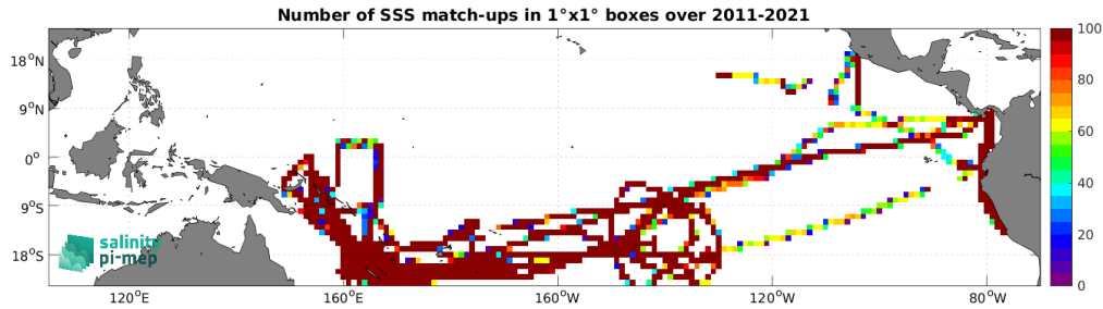
Figure 5: Number of SSS match-ups between TSG (GOSUD-Research-vessel) SSS and the SMOS SSS L4 v2 - Daily (BEC) SSS product for the Tropical Pacific Ocean Pi-MEP region over 1^\circ \times 1^\circ boxes and for the full satellite product period.
