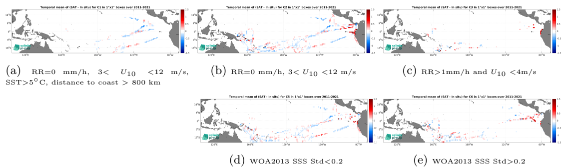
Figure 14: Temporal mean gridded over spatial boxes of size 1^\circ \times 1^\circ of \Delta SSS (SMOS SSS L4 v2 - Daily (BEC) - TSG (GOSUD-Research-vessel)) for 5 different subdatasets corresponding to: RR=0 mm/h, 3 < U_{10} < 12 m/s, SST > 5°C, distance to coast > 800 km (a), RR=0 mm/h, 3 < U_{10} < 12 m/s (b), RR > 1mm/h and U_{10} < 4 m/s (c), WOA2013 SSS Std < 0.2 (d), WOA2013 SSS Std > 0.2 (e).
