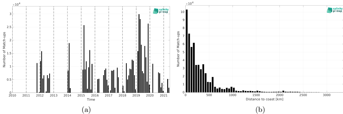
Figure 2: Number of match-ups between TSG (GOSUD-Research-vessel) and SMOS SSS L4 v2 - Daily (BEC) SSS as a function of time (a) and as function of the distance to coast (b) over the Tropical Pacific Ocean Pi-MEP region and for the full satellite product period.
