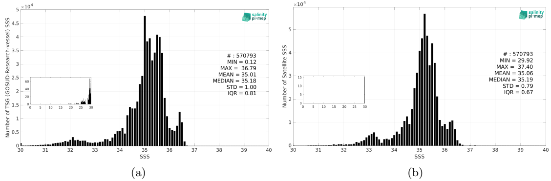
Figure 3: Histograms of SSS from TSG (GOSUD-Research-vessel) (a) and SMOS SSS L4 v2 - Daily (BEC) (b) considering all match-up pairs per bins of 0.1 over the Tropical Pacific Ocean Pi-MEP region and for the full satellite product period.
