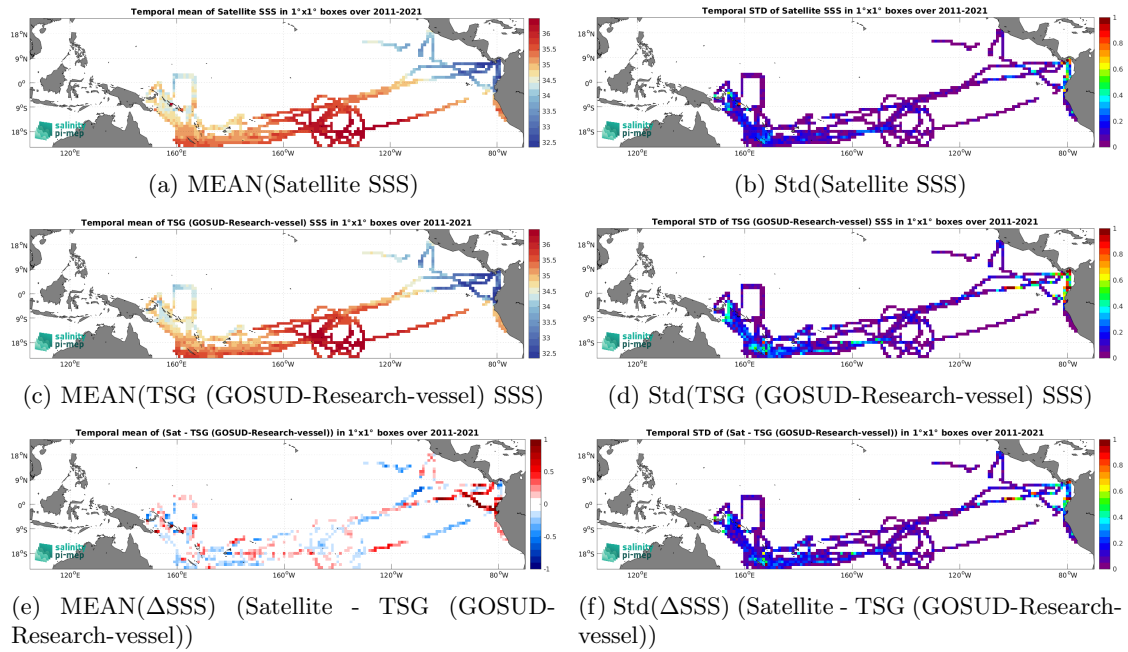
Figure 7: Temporal mean (left) and Std (right) of SSS from SMOS SSS L4 v2 - Daily (BEC) (top), TSG (GOSUD-Research-vessel) (middle), and of \Delta SSS (Satellite - TSG (GOSUD-Research-vessel)). Only match-up pairs are used to generate these maps.
