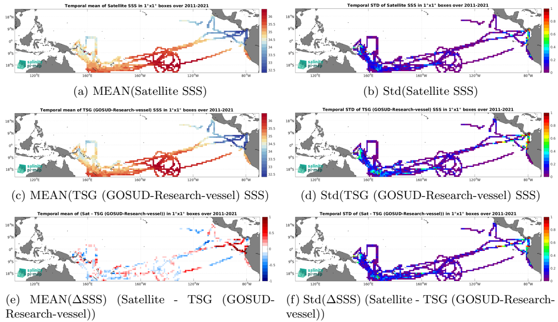
Figure 6: Temporal mean (left) and Std (right) of SSS from SMOS SSS L4 v2 - Daily (BEC) (top), TSG (GOSUD-Research-vessel) (middle), and of \Delta SSS (Satellite - TSG (GOSUD-Research-vessel)). Only match-up pairs are used to generate these maps.
