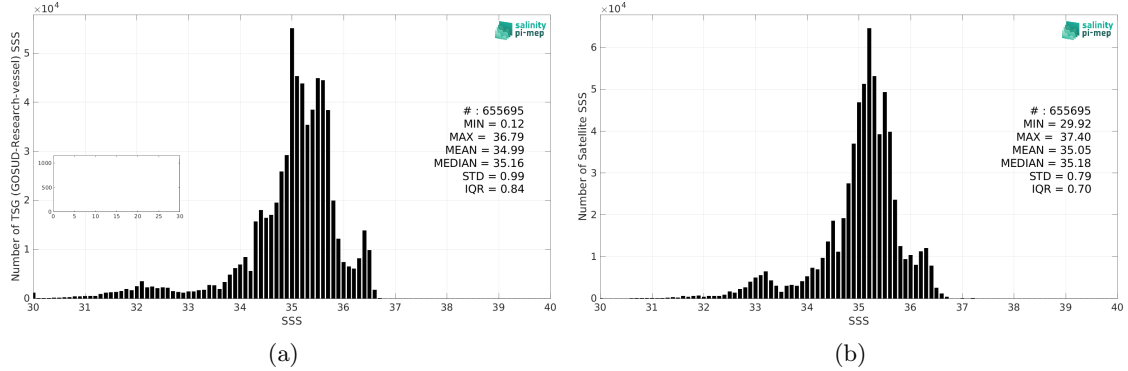
Figure 2: Histograms of SSS from TSG (GOSUD-Research-vessel) (a) and SMOS SSS L4 v2 - Daily (BEC) (b) considering all match-up pairs per bins of 0.1 over the Tropical Pacific Ocean Pi-MEP region and for the full satellite product period.
