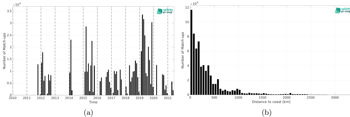
Figure 1: Number of match-ups between TSG (GOSUD-Research-vessel) and SMOS SSS L4 v2 - Daily (BEC) SSS as a function of time (a) and as function of the distance to coast (b) over the Tropical Pacific Ocean Pi-MEP region and for the full satellite product period.
