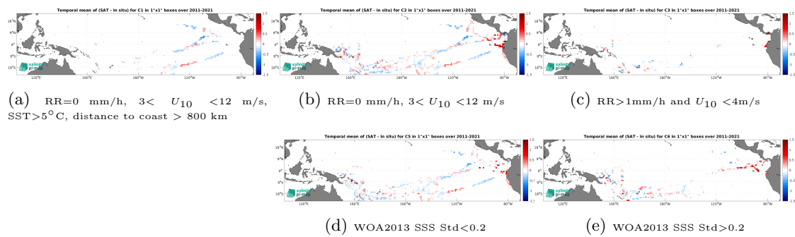
Figure 12: Temporal mean gridded over spatial boxes of size 1^\circ \times 1^\circ of \Delta SSS (SMOS SSS L4 v2 - Daily (BEC) - TSG (GOSUD-Research-vessel)) for 5 different subdatasets corresponding to:RR=0 mm/h, 3 < U_{10} < 12 m/s, SST >5^\circ\text{C} , distance to coast > 800 km (a), RR=0 mm/h, 3 < U_{10} < 12 m/s (b), RR >1 mm/h and U_{10} < 4 m/s (c), WOA2013 SSS Std <0.2 (d), WOA2013 SSS Std >0.2 (e).
