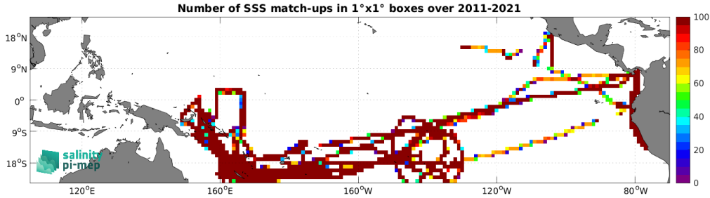
Figure 4: Number of SSS match-ups between TSG (GOSUD-Research-vessel) SSS and the SMOS SSS L4 v2 - Daily (BEC) SSS product for the Tropical Pacific Ocean Pi-MEP region over 1^\circ \times 1^\circ boxes and for the full satellite product period.
