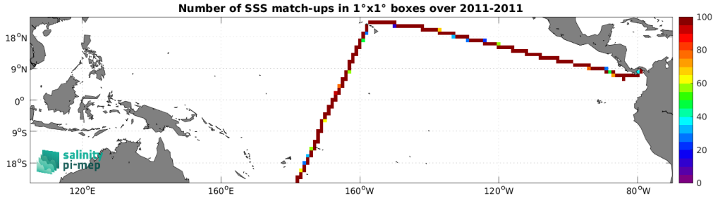
Figure 5: Number of SSS match-ups between TSG (CSIC-UTM) SSS and the SMOS SSS L4 v2 - Daily (BEC) SSS product for the Tropical Pacific Ocean Pi-MEP region over 1^\circ \times 1^\circ boxes and for the full satellite product period.
