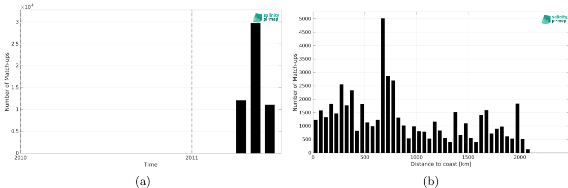
Figure 2: Number of match-ups between TSG (CSIC-UTM) and SMOS SSS L4 v2 - Daily (BEC) SSS as a function of time (a) and as function of the distance to coast (b) over the Tropical Pacific Ocean Pi-MEP region and for the full satellite product period.
