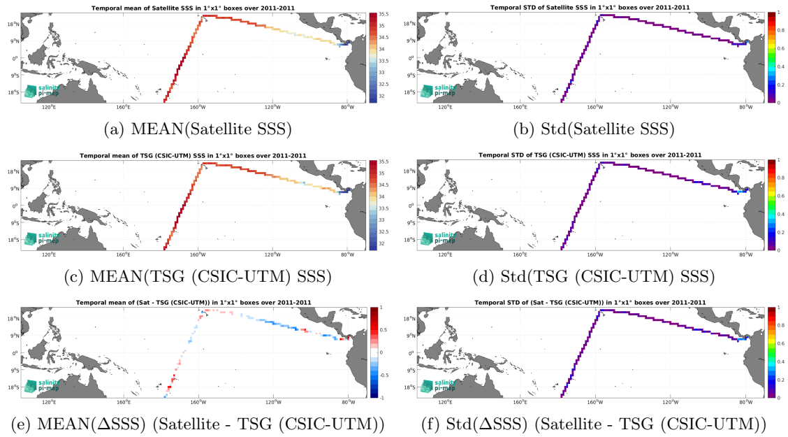
Figure 7: Temporal mean (left) and Std (right) of SSS from SMOS SSS L4 v2 - Daily (BEC) (top), TSG (CSIC-UTM) (middle), and of \Delta SSS (Satellite - TSG (CSIC-UTM)). Only match-up pairs are used to generate these maps.
