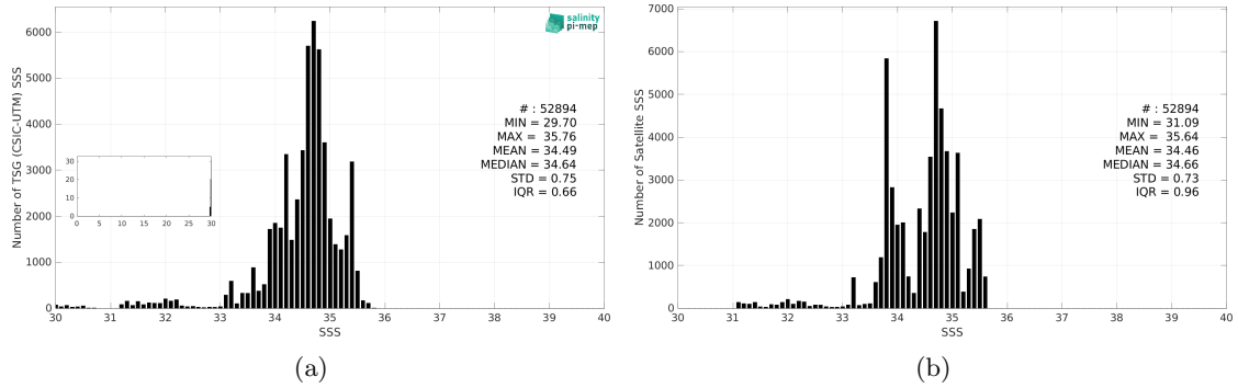
Figure 3: Histograms of SSS from TSG (CSIC-UTM) (a) and SMOS SSS L4 v2 - Daily (BEC) (b) considering all match-up pairs per bins of 0.1 over the Tropical Pacific Ocean Pi-MEP region and for the full satellite product period.
