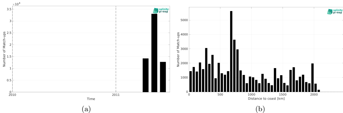
Figure 1: Number of match-ups between TSG (CSIC-UTM) and SMOS SSS L4 v2 - Daily (BEC) SSS as a function of time (a) and as function of the distance to coast (b) over the Tropical Pacific Ocean Pi-MEP region and for the full satellite product period.
