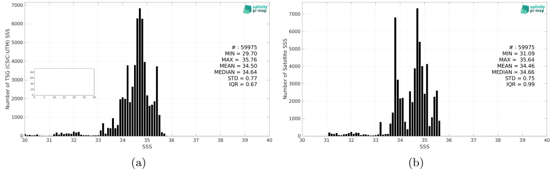
Figure 2: Histograms of SSS from TSG (CSIC-UTM) (a) and SMOS SSS L4 v2 - Daily (BEC) (b) considering all match-up pairs per bins of 0.1 over the Tropical Pacific Ocean Pi-MEP region and for the full satellite product period.
