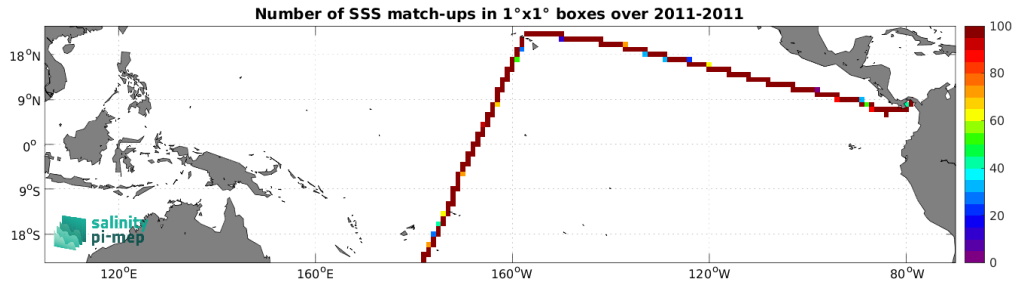
Figure 4: Number of SSS match-ups between TSG (CSIC-UTM) SSS and the SMOS SSS L4 v2 - Daily (BEC) SSS product for the Tropical Pacific Ocean Pi-MEP region over 1^\circ \times 1^\circ boxes and for the full satellite product period.
