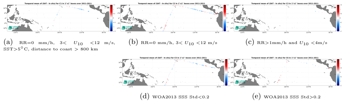
Figure 12: Temporal mean gridded over spatial boxes of size 1^\circ \times 1^\circ of \Delta SSS (SMOS SSS L4 v2 - Daily (BEC) - TSG (CSIC-UTM)) for 5 different subdatasets corresponding to: RR=0 mm/h, 3 < U_{10} < 12 m/s, SST > 5^\circ\text{C} , distance to coast > 800 km (a), RR=0 mm/h, 3 < U_{10} < 12 m/s (b), RR > 1 mm/h and U_{10} < 4 m/s (c), WOA2013 SSS Std < 0.2 (d), WOA2013 SSS Std > 0.2 (e).
