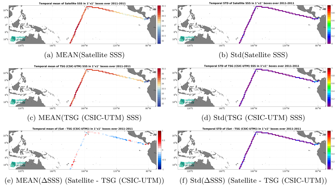
Figure 6: Temporal mean (left) and Std (right) of SSS from SMOS SSS L4 v2 - Daily (BEC) (top), TSG (CSIC-UTM) (middle), and of \Delta SSS (Satellite - TSG (CSIC-UTM)). Only match-up pairs are used to generate these maps.
