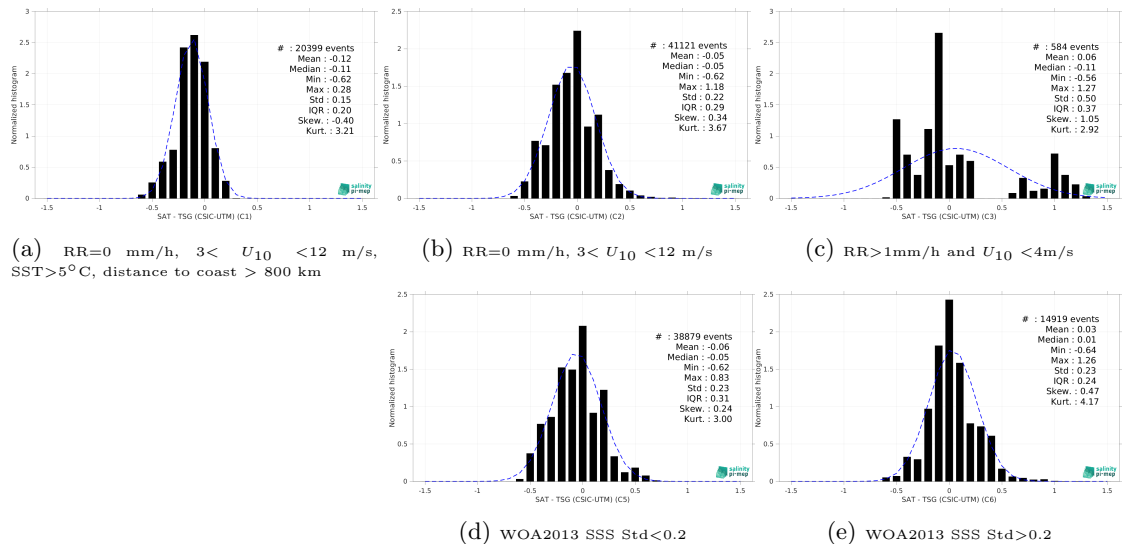
Figure 13: Normalized histogram of \Delta SSS (SMOS SSS L4 v2 - Daily (BEC) - TSG (CSIC-UTM)) for 5 different subdatasets corresponding to: RR=0 mm/h, 3 < U_{10} < 12 m/s, SST > 5^\circ\text{C} , distance to coast > 800 km (a), RR=0 mm/h, 3 < U_{10} < 12 m/s (b), RR > 1 mm/h and U_{10} < 4 m/s (c), WOA2013 SSS Std < 0.2 (d), WOA2013 SSS Std > 0.2 (e).
