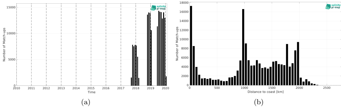
Figure 2: Number of match-ups between Saildrone and SMOS SSS L4 v2 - Daily (BEC) SSS as a function of time (a) and as function of the distance to coast (b) over the Tropical Pacific Ocean Pi-MEP region and for the full satellite product period.
