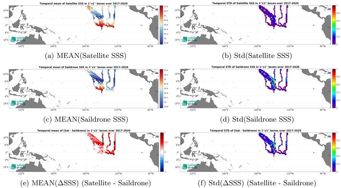
Figure 7: Temporal mean (left) and Std (right) of SSS from SMOS SSS L4 v2 - Daily (BEC) (top), Saildrone (middle), and of \Delta SSS (Satellite - Saildrone). Only match-up pairs are used to generate these maps.
