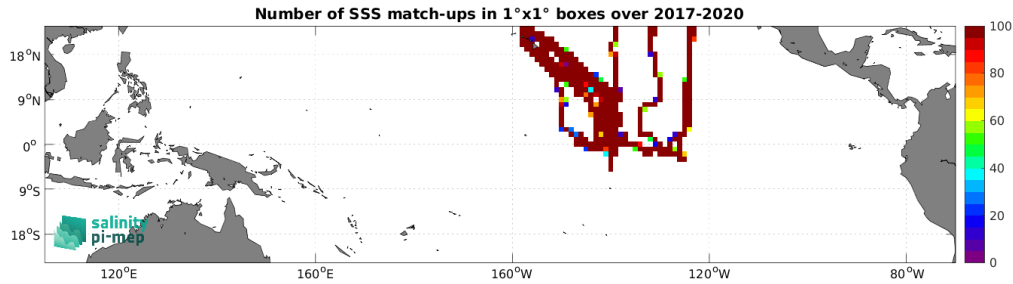
Figure 5: Number of SSS match-ups between Saildrone SSS and the SMOS SSS L4 v2 - Daily (BEC) SSS product for the Tropical Pacific Ocean Pi-MEP region over 1^\circ \times 1^\circ boxes and for the full satellite product period.
