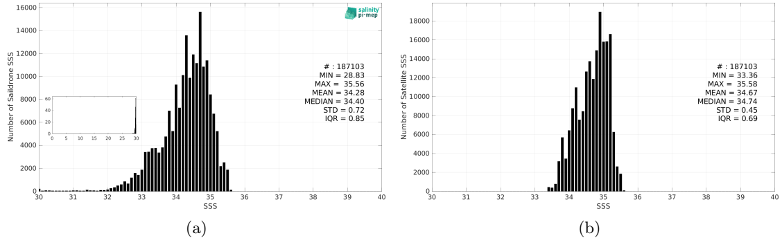
Figure 3: Histograms of SSS from Saildrone (a) and SMOS SSS L4 v2 - Daily (BEC) (b) considering all match-up pairs per bins of 0.1 over the Tropical Pacific Ocean Pi-MEP region and for the full satellite product period.
