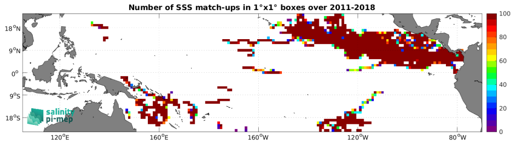
Figure 4: Number of SSS match-ups between Surface drifters SSS and the SMOS SSS L4 v2 - Daily (BEC) SSS product for the Tropical Pacific Ocean Pi-MEP region over 1^\circ \times 1^\circ boxes and for the full satellite product period.
