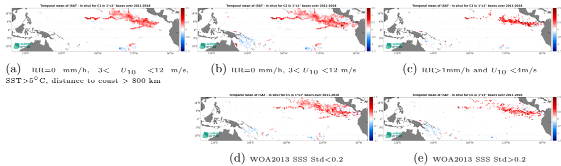
Figure 13: Temporal mean gridded over spatial boxes of size 1^\circ \times 1^\circ of \Delta\text{SSS} (SMOS SSS L4 v2 - Daily (BEC) - Surface drifters) for 5 different subdatasets corresponding to: RR=0 mm/h, 3 < U_{10} < 12 m/s, SST >5^\circ\text{C} , distance to coast > 800 km (a), RR=0 mm/h, 3 < U_{10} < 12 m/s (b), RR >1 mm/h and U_{10} < 4 m/s (c), WOA2013 SSS Std <0.2 (d), WOA2013 SSS Std >0.2 (e).
