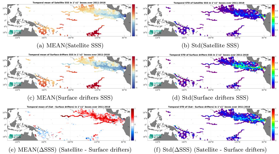
Figure 6: Temporal mean (left) and Std (right) of SSS from SMOS SSS L4 v2 - Daily (BEC) (top), Surface drifters (middle), and of \Delta SSS (Satellite - Surface drifters). Only match-up pairs are used to generate these maps.
