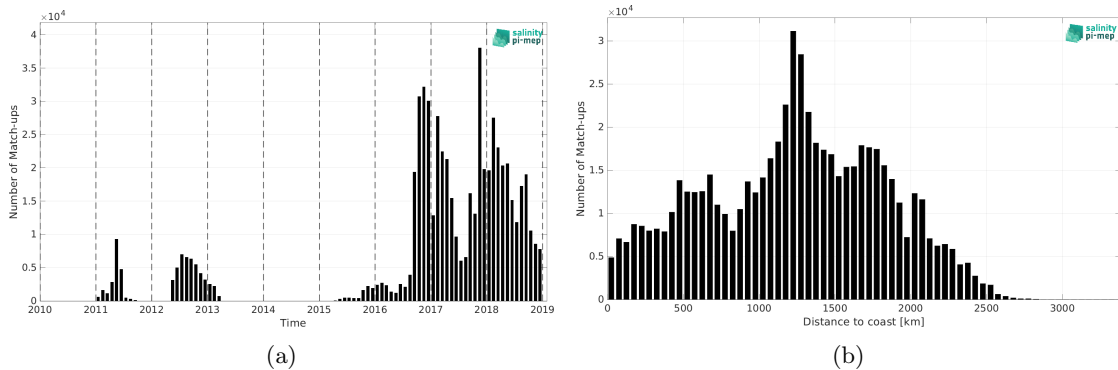
Figure 2: Number of match-ups between Surface drifters and SMOS SSS L4 v2 - Daily (BEC) SSS as a function of time (a) and as function of the distance to coast (b) over the Tropical Pacific Ocean Pi-MEP region and for the full satellite product period.
