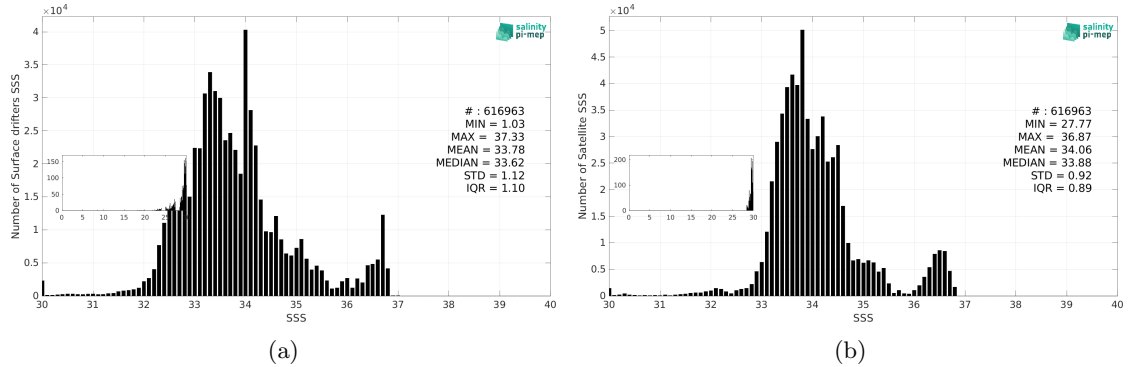
Figure 3: Histograms of SSS from Surface drifters (a) and SMOS SSS L4 v2 - Daily (BEC) (b) considering all match-up pairs per bins of 0.1 over the Tropical Pacific Ocean Pi-MEP region and for the full satellite product period.
