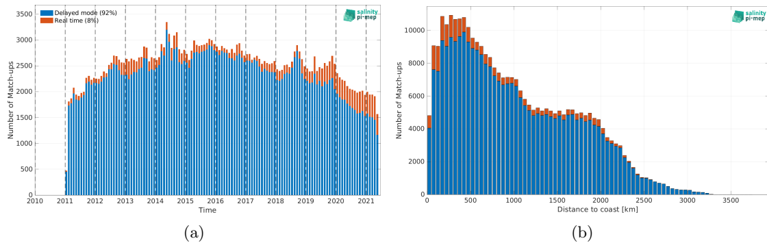
Figure 1: Number of match-ups between Argo and SMOS SSS L4 v2 - Daily (BEC) SSS as a function of time (a) and as function of the distance to coast (b) over the Tropical Pacific Ocean Pi-MEP region and for the full satellite product period.
