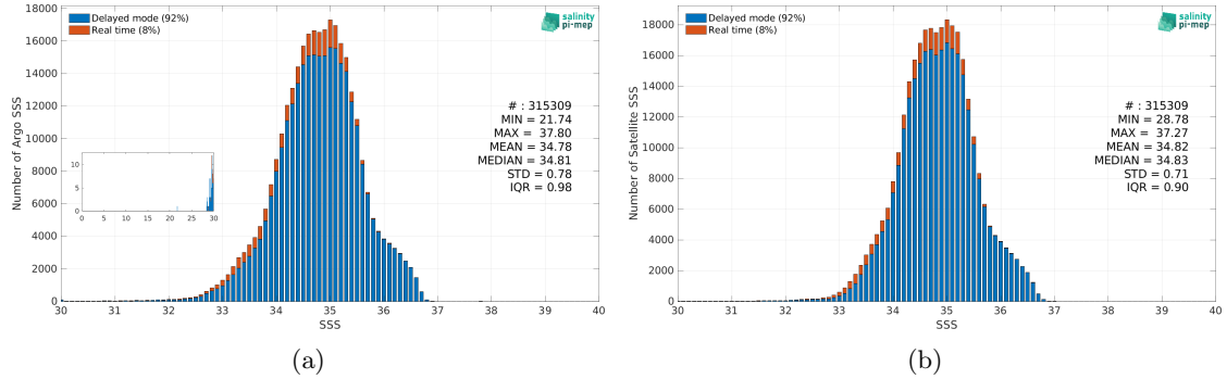
Figure 2: Histograms of SSS from Argo (a) and SMOS SSS L4 v2 - Daily (BEC) (b) considering all match-up pairs per bins of 0.1 over the Tropical Pacific Ocean Pi-MEP region and for the full satellite product period.
