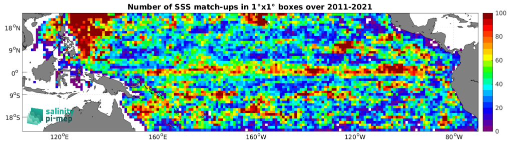
Figure 4: Number of SSS match-ups between Argo SSS and the SMOS SSS L4 v2 - Daily (BEC) SSS product for the Tropical Pacific Ocean Pi-MEP region over 1^\circ \times 1^\circ boxes and for the full satellite product period.
