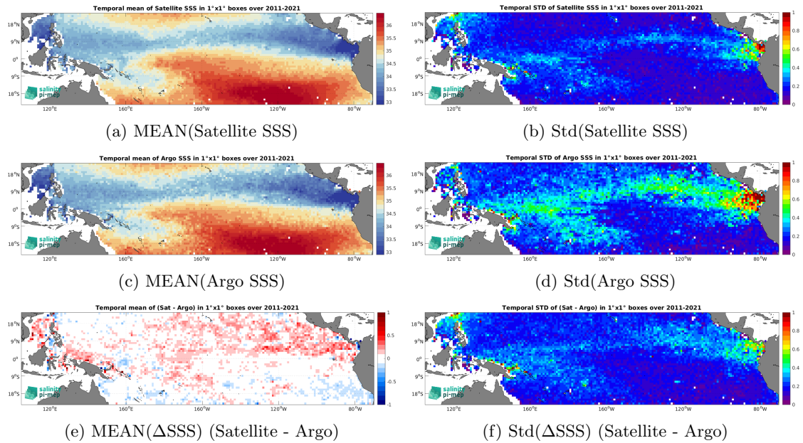
Figure 6: Temporal mean (left) and Std (right) of SSS from SMOS SSS L4 v2 - Daily (BEC) (top), Argo (middle), and of \Delta SSS (Satellite - Argo). Only match-up pairs are used to generate these maps.
