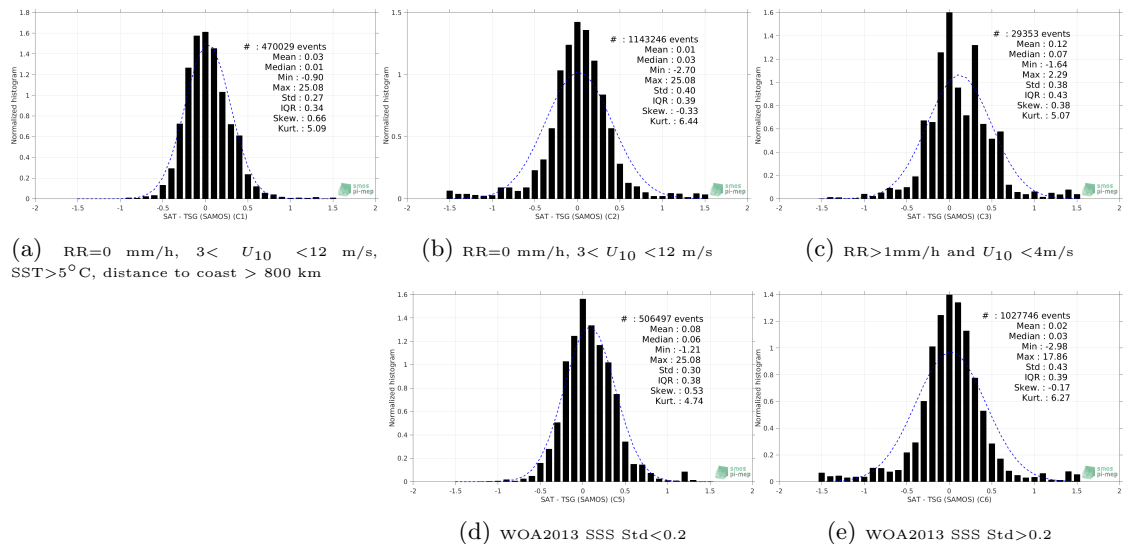
Figure 13: Normalized histogram of \Delta SSS (SMOS SSS L3 v3 Monthly (ICDC) - TSG (SAMOS)) for 5 different subdatasets corresponding to: RR=0 mm/h, 3 < U_{10} < 12 m/s, SST >5^\circ\text{C} , distance to coast > 800 km (a), RR=0 mm/h, 3 < U_{10} < 12 m/s (b), RR >1 mm/h and U_{10} < 4 m/s (c), WOA2013 SSS Std <0.2 (d), WOA2013 SSS Std >0.2 (e).
