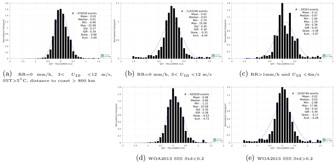
Figure 13: Normalized histogram of \Delta SSS (SMOS-L3-ICDC-V3-MONTHLY-0.5DEG - TSG-SAMOS) for 5 different subdatasets corresponding to: RR=0 mm/h, 3 < U_{10} < 12 m/s, SST > 5°C, distance to coast > 800 km (a), RR=0 mm/h, 3 < U_{10} < 12 m/s (b), RR > 1mm/h and U_{10} < 4m/s (c), WOA2013 SSS Std < 0.2 (d), WOA2013 SSS Std > 0.2 (e).
