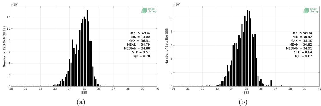
Figure 2: Histograms of SSS from TSG-SAMOS (a) and SMOS-L3-ICDC-V3-MONTHLY-0.5DEG (b) considering all match-up pairs per bins of 0.1 over the Tropical Pacific Ocean Pi-MEP region and for the full satellite product period.
