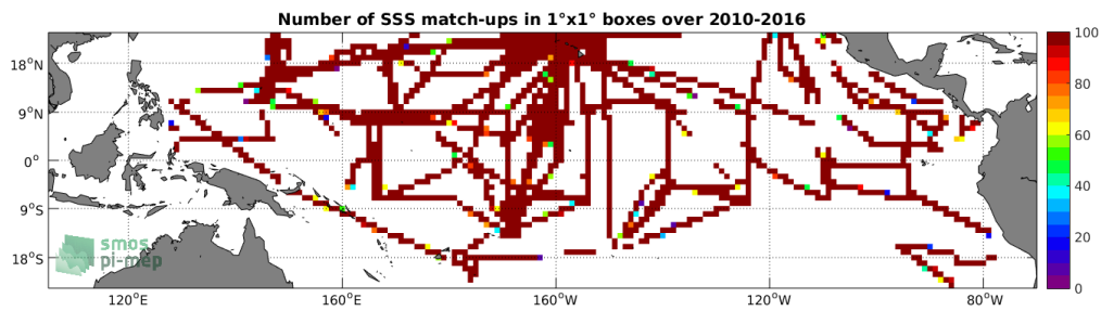
Figure 4: Number of SSS match-ups between TSG-SAMOS SSS and the SMOS-L3-ICDC-V3-MONTHLY-0.5DEG SSS product for the Tropical Pacific Ocean Pi-MEP region over 1^\circ \times 1^\circ boxes and for the full satellite product period.
