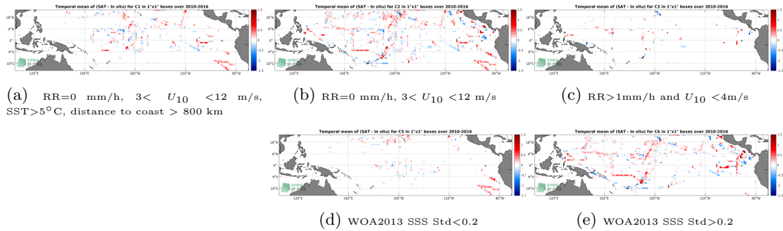
Figure 12: Temporal mean gridded over spatial boxes of size 1°x1° of \Delta SSS (SMOS-L3-ICDC-V3-MONTHLY-0.5DEG - TSG-SAMOS) for 5 different subdatasets corresponding to:RR=0 mm/h, 3 < U_{10} < 12 m/s, SST > 5°C, distance to coast > 800 km (a), RR=0 mm/h, 3 < U_{10} < 12 m/s (b), RR > 1mm/h and U_{10} < 4m/s (c), WOA2013 SSS Std < 0.2 (d), WOA2013 SSS Std > 0.2 (e).
