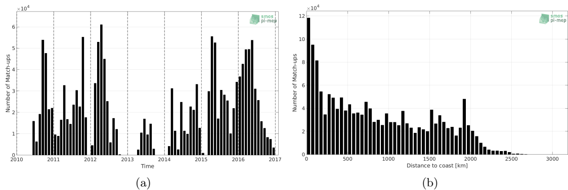
Figure 1: Number of match-ups between TSG-SAMOS and SMOS-L3-ICDC-V3-MONTHLY-0.5DEG SSS as a function of time (a) and as function of the distance to coast (b) over the Tropical Pacific Ocean Pi-MEP region and for the full satellite product period.
