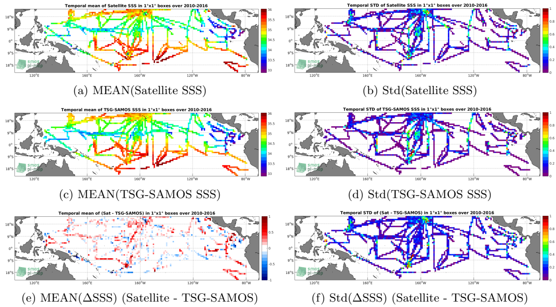
Figure 6: Temporal mean (left) and Std (right) of SSS from SMOS-L3-ICDC-V3-MONTHLY-0.5DEG (top), TSG-SAMOS (middle), and of \Delta SSS (Satellite - TSG-SAMOS). Only match-up pairs are used to generate these maps.
